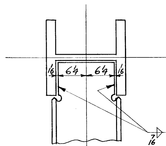
TYPICAL WEB CONN. FOR DIAGONAL MEMBERS Wg & Wh
