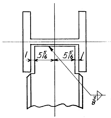
TYPICAL WEB CONN. FOR VERTICAL MEMBERS Wm & Wn
