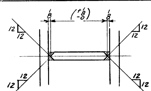
SECTION K-K
