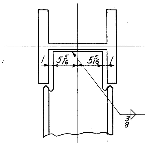
TYPICAL WEB CONN. FOR VERTICAL MEMBERS WK
