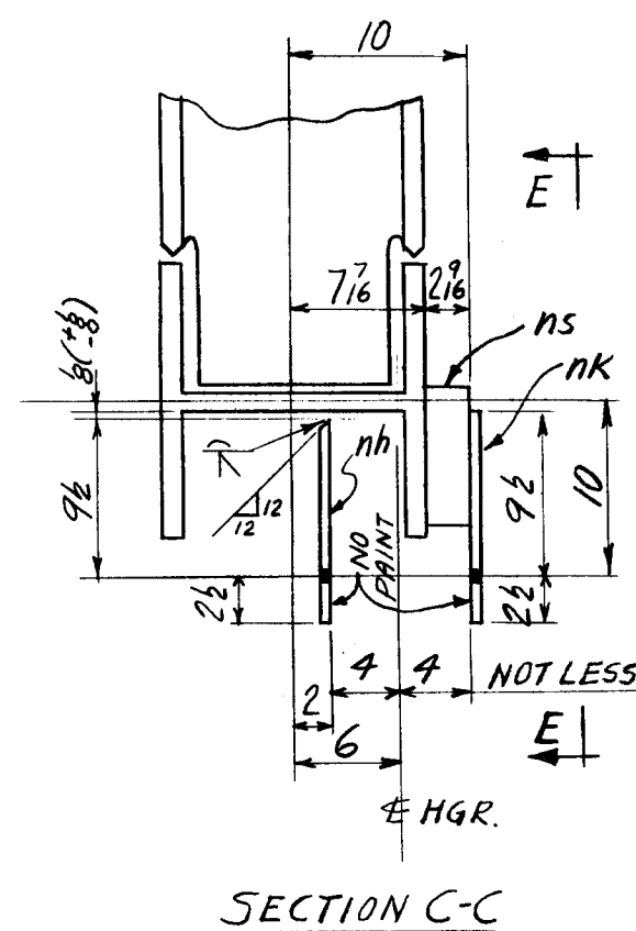
SECTION C-C
