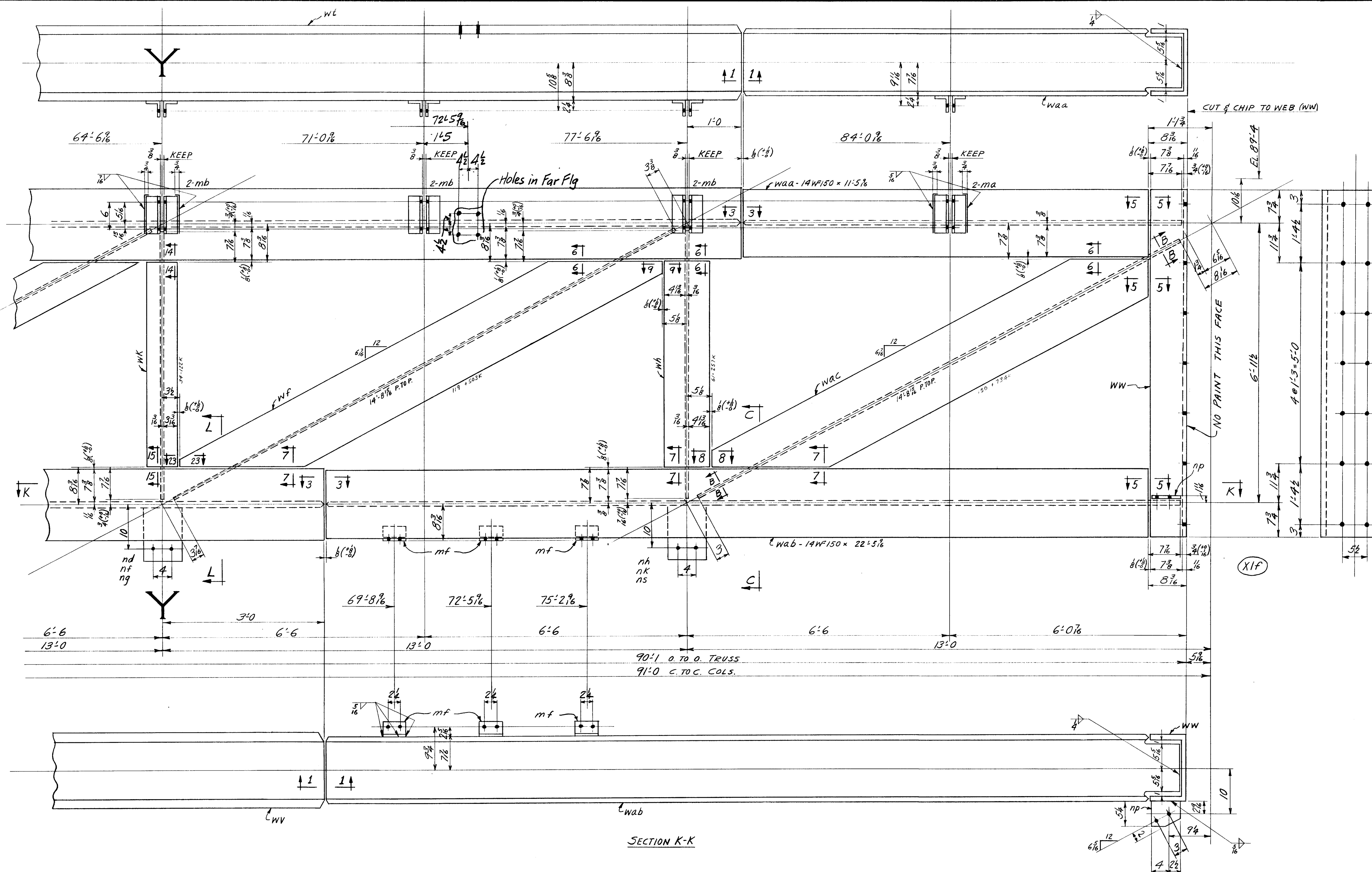
ONE TRUSS MK. BT8
