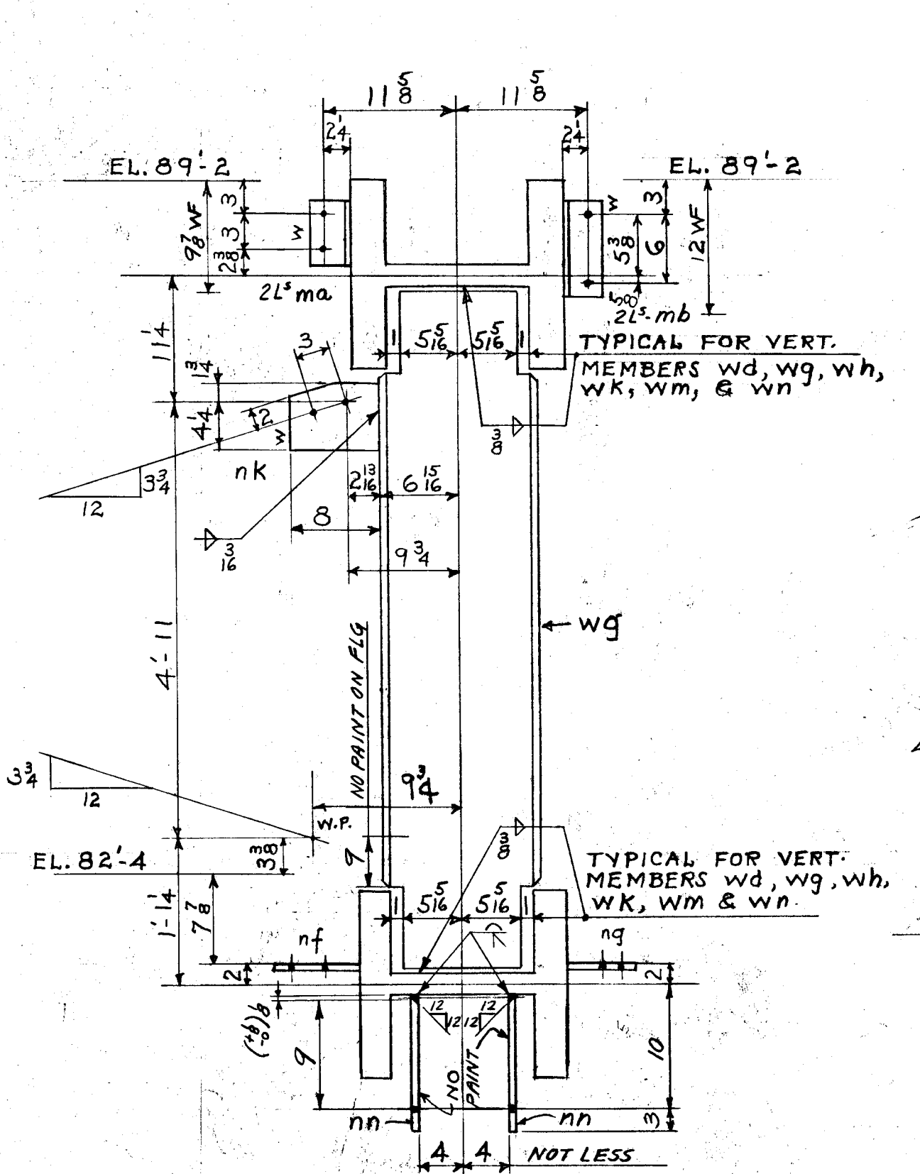
SECTION B-B FOR TRUSS T7
