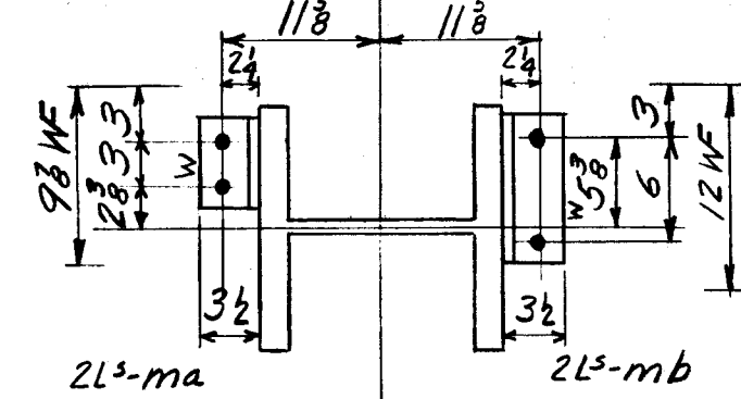
SECTION C-C FOR TRUSS T7
