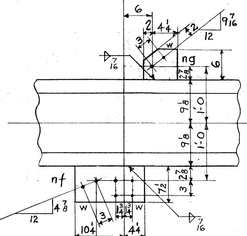
SECTION D-D FOR TRUSS T7
