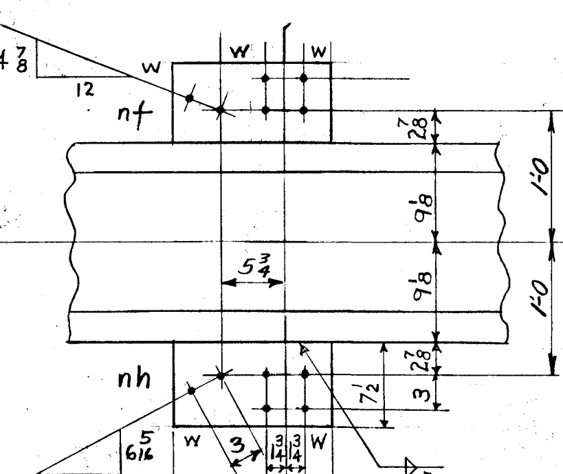
SECTION D-D FOR TRUSS T7A
