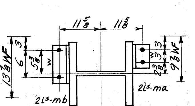
SECTION C-C FOR TRUSS T7A
