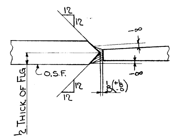
SECTION 19-19
