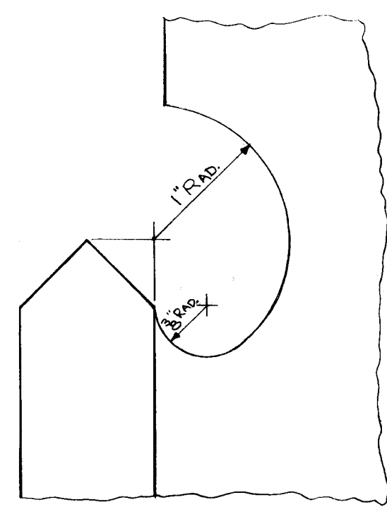
TYPICAL DETAIL FOR BURNING WEBS OF DIAGONALS 14W43 AND OVER
