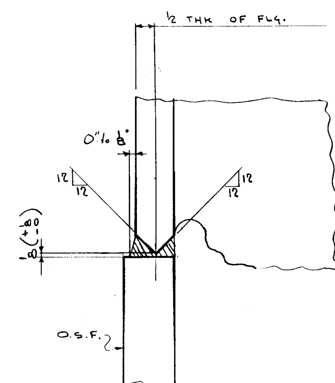
SECTION 7-7
