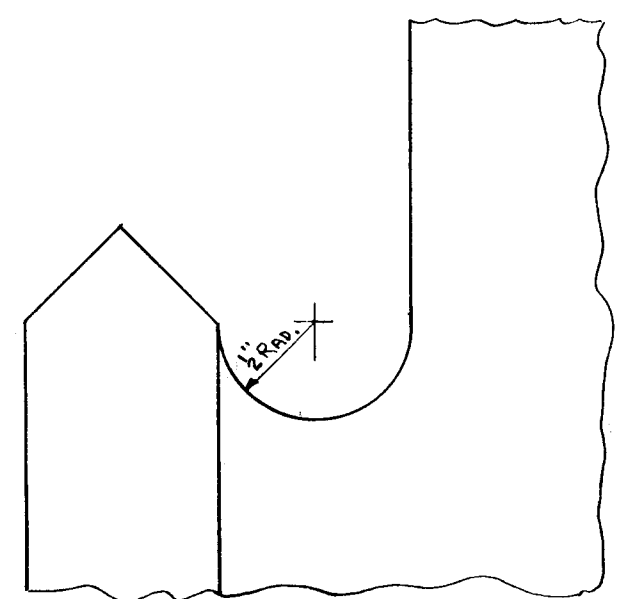
TYPICAL DETAIL FOR BURNING WEBS OF VERTICALS, TOP & BOTTOM CHORD MEMBERS 14W43 AND OVER
