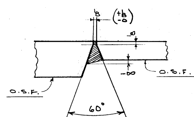
SECTION 3-3
