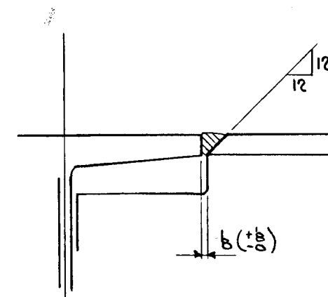
DETAIL "A" Typical for Sect. 13-13
