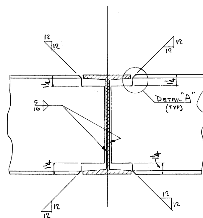
SECTION 13-13
