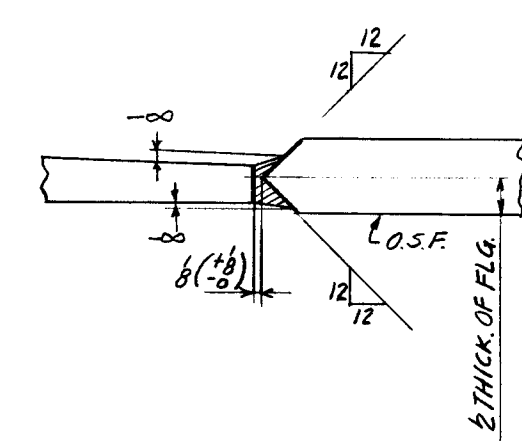
SECTION 23-23
