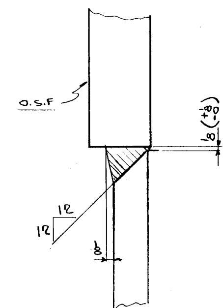
SECTION 14-14
