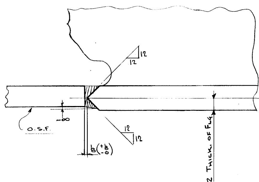
SECTION 8-8
