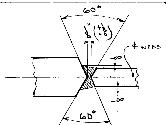
TYPICAL DETAIL FOR BURNING WEBS OF VERTICALS, TOP & BOTTOM CHORD MEMBERS 14W43 AND OVER
