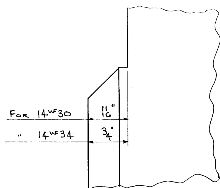
TYPICAL DETAIL FOR BURNING WEBS OF DIAGONALS OF 14W30 AND 14W34
