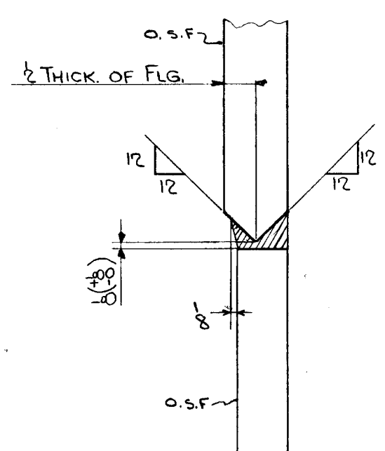
SECTION 16-16
