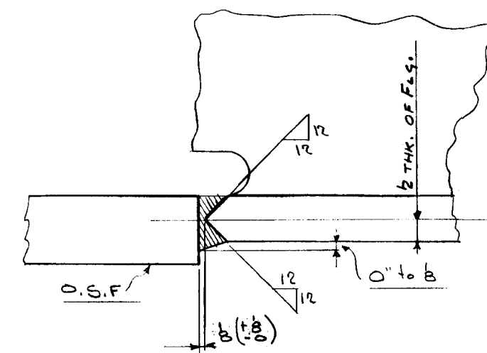
SECTION 4-4
