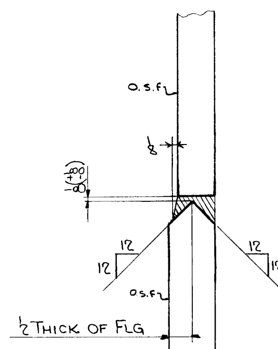
SECTION 17-17
