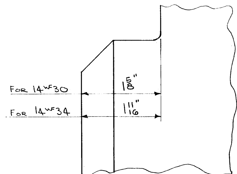
TYPICAL DETAIL FOR BURNING WEBS OF DIAGONALS OF 14W30 AND 14W34
