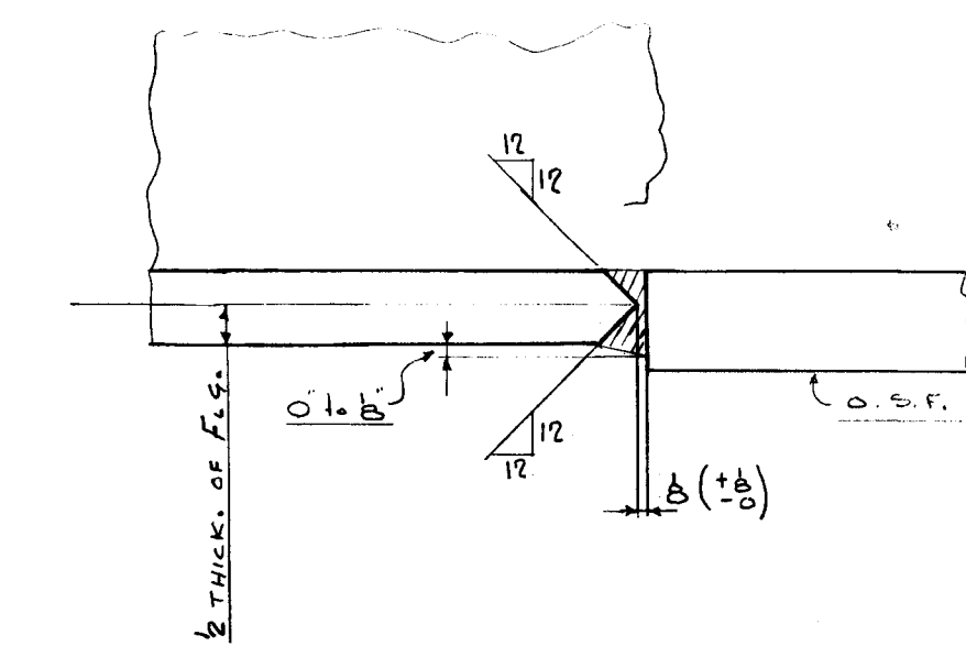
SECTION 5-5
