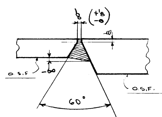
SECTION 10-10
