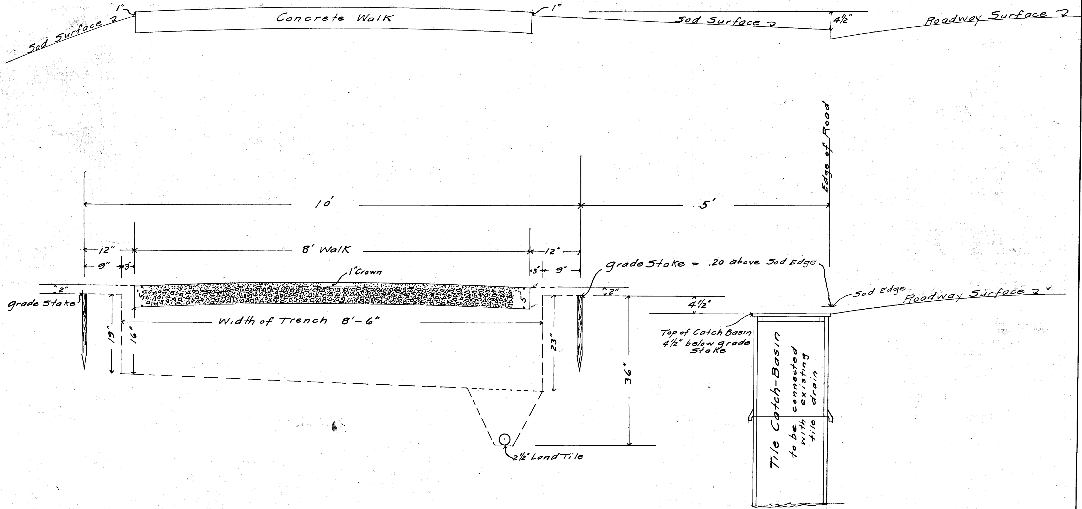
Cross Section Pope Park Walk Scale - One Inch = One Foot
