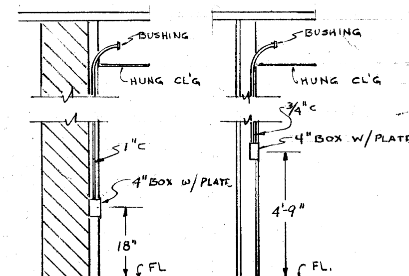
TELEPHONE OUTLET DETAIL NO SCALE
