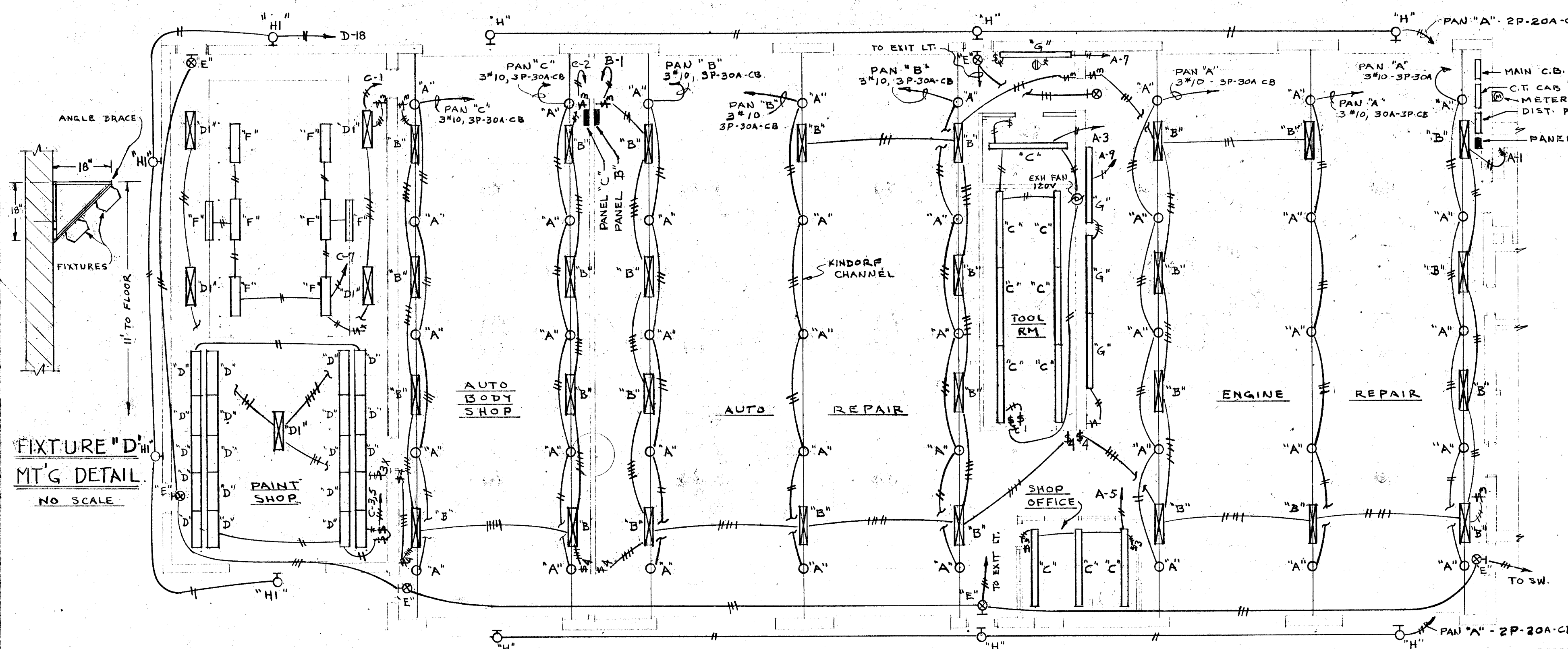
LIGHTING PLAN SCALE 1/8" = 1'-0"
