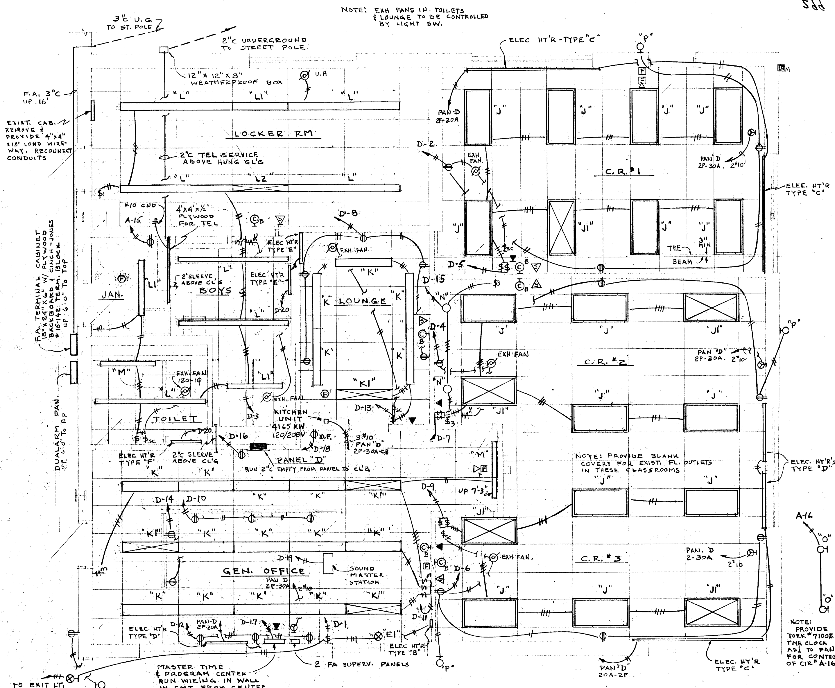
LIGHTING-POWER-SIGNAL PLAN SCALE 1/4" = 1'-0"
