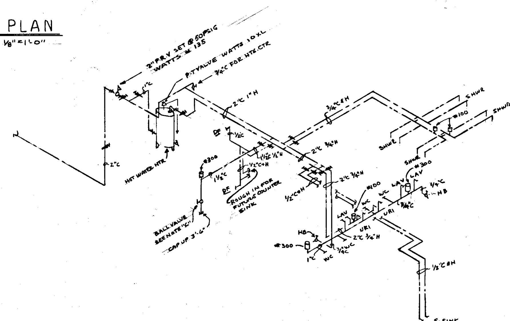
SCHEMATIC WATER PIPING
