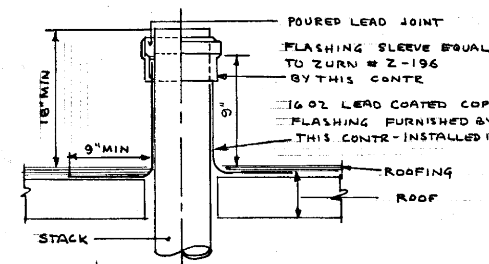
TYPICAL VENT FLASHING DETAIL
