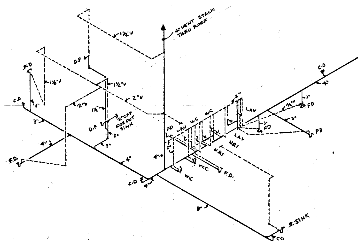
SCHEMATIC WASTE & VENT PIPING
