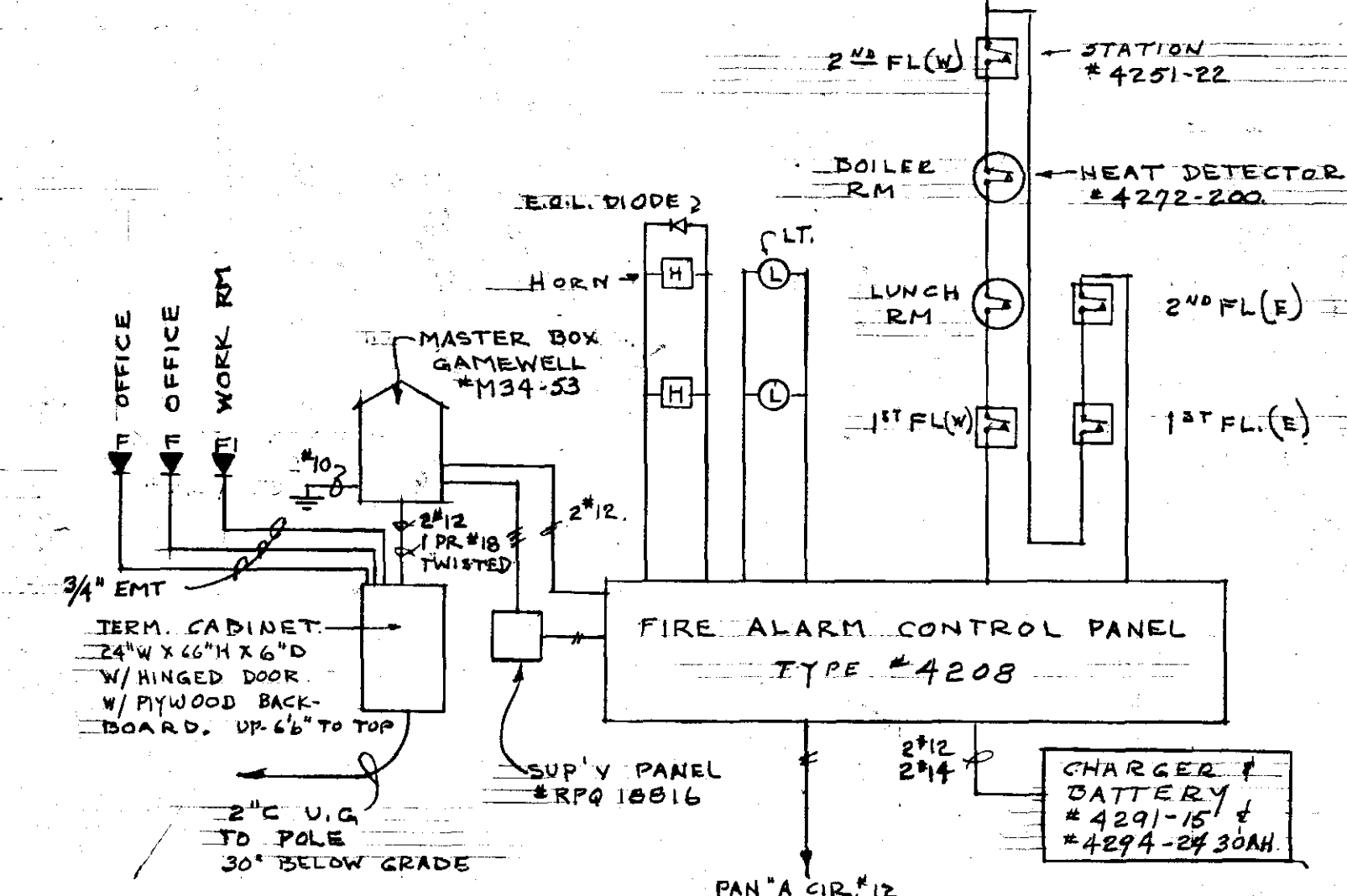
FIRE ALARM RISER DIAGRAM
