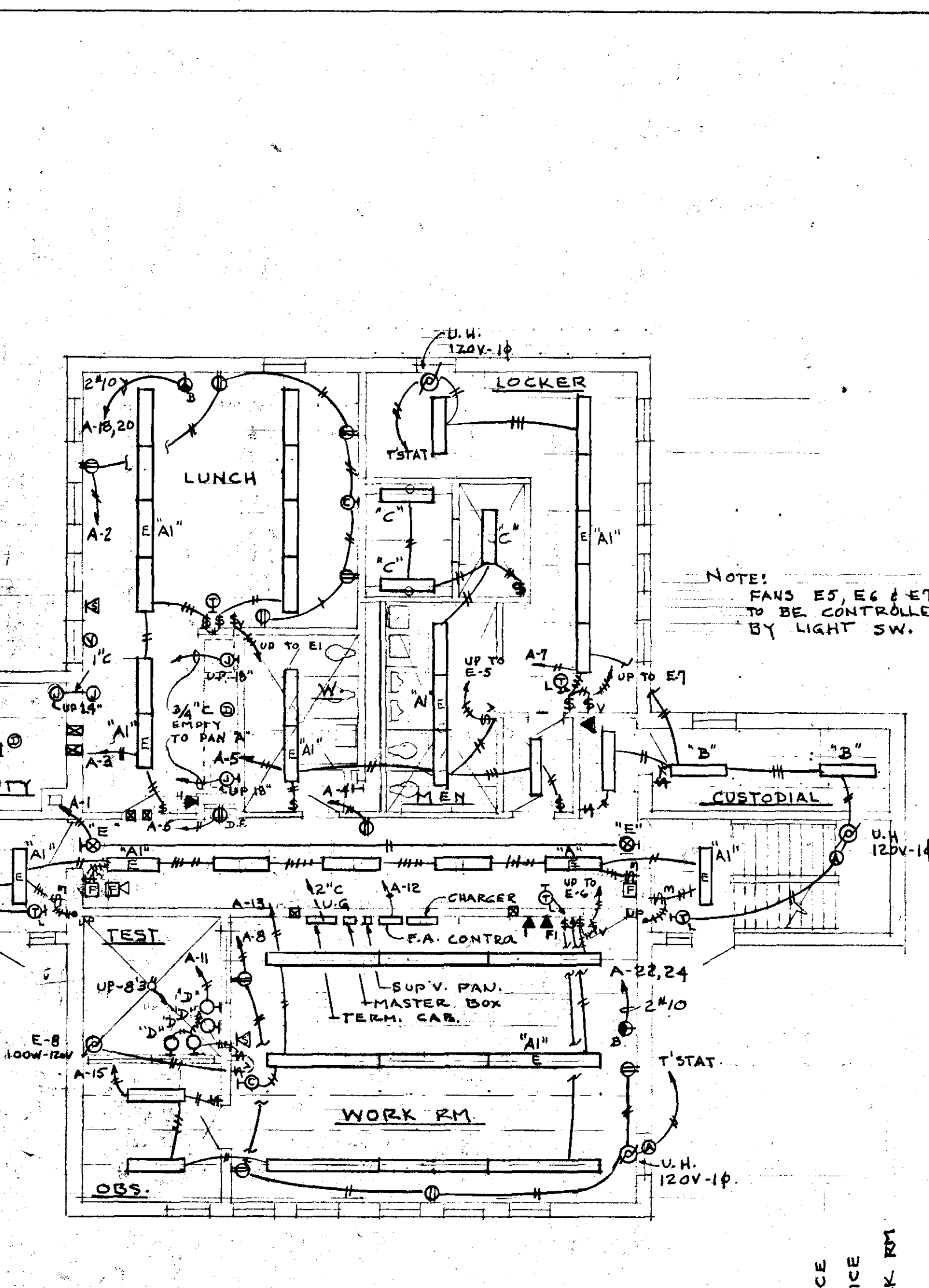
FIRST FLOOR PLAN SCALE 1/8" = 1'-0"
