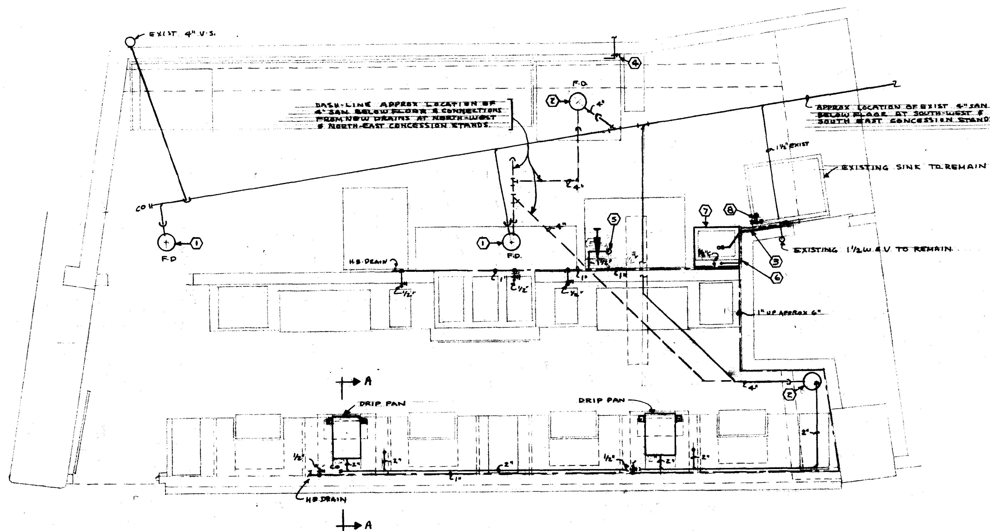
PLUMBING PLAN RE & S.W. CONCESSIONS SCALE 1/2" = 1'-0" (N.W. & S.E. CONCESSIONS HAVE REVERSED FLOOR PLANS)
