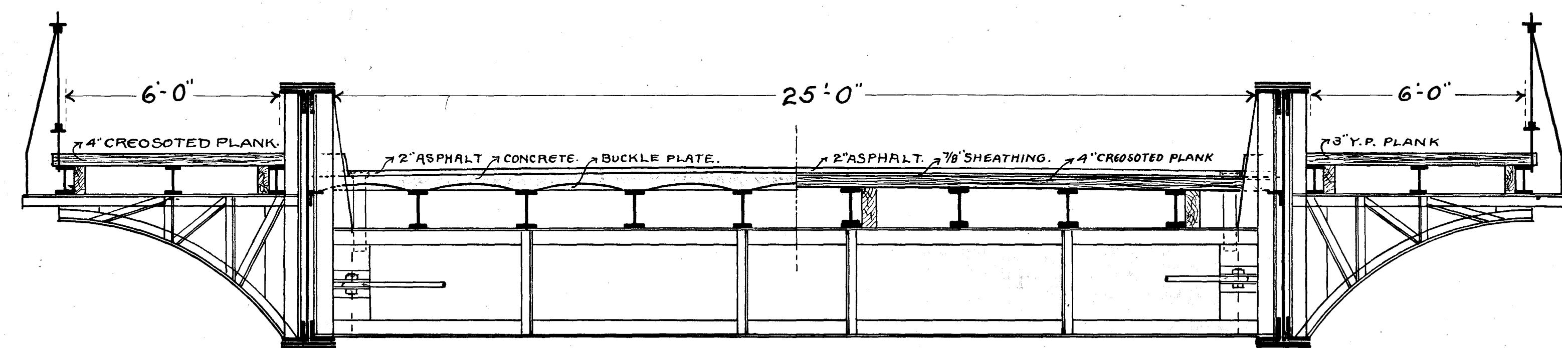
CROSS SECTION.
