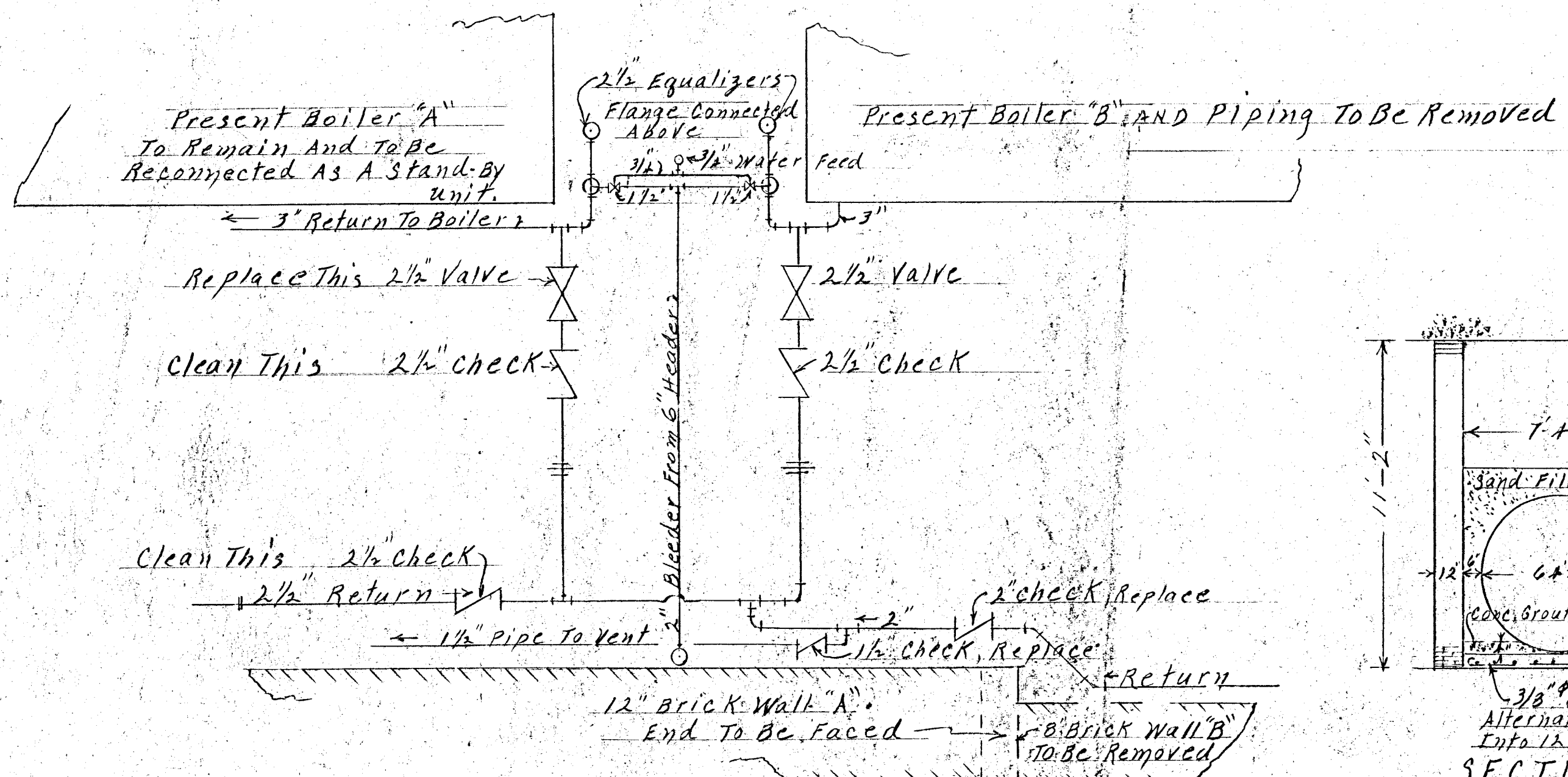
DETAIL OF PRESENT BOILER RETURN CONNECTIONS SCALE ABOUT 1" = 1'
