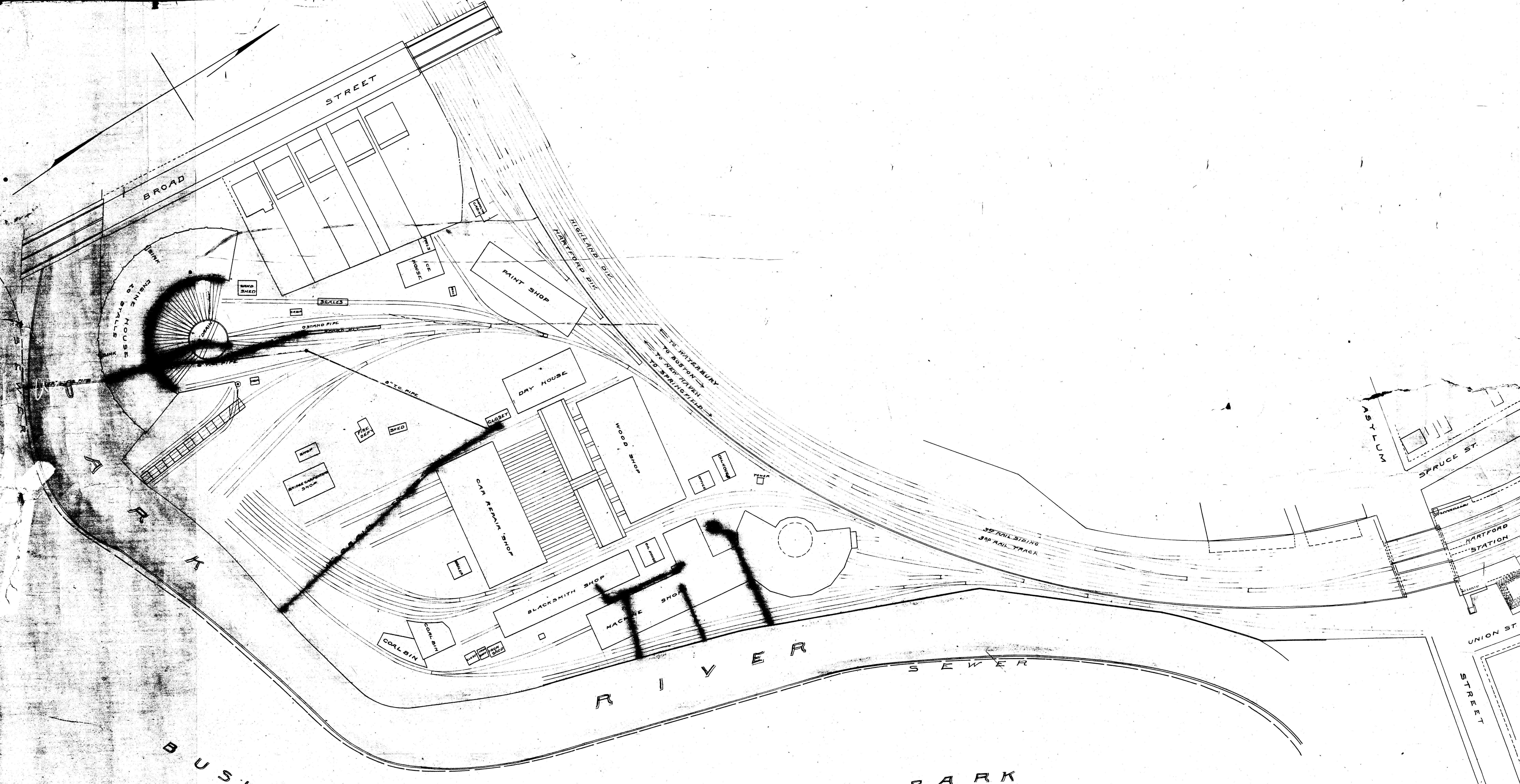
MAP SHOWING PROPOSED SEWER HARTFORD SHOPS HARTFORD, CONN. HARTFORD DIV. N.Y. N.H. & H.R.R. SCALE 1"=50' NOV., 1904
