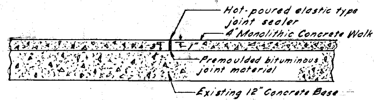
SECTION OF WALK AND DETAIL OF JOINT SCALE \frac{1}{2}'' = 1'
