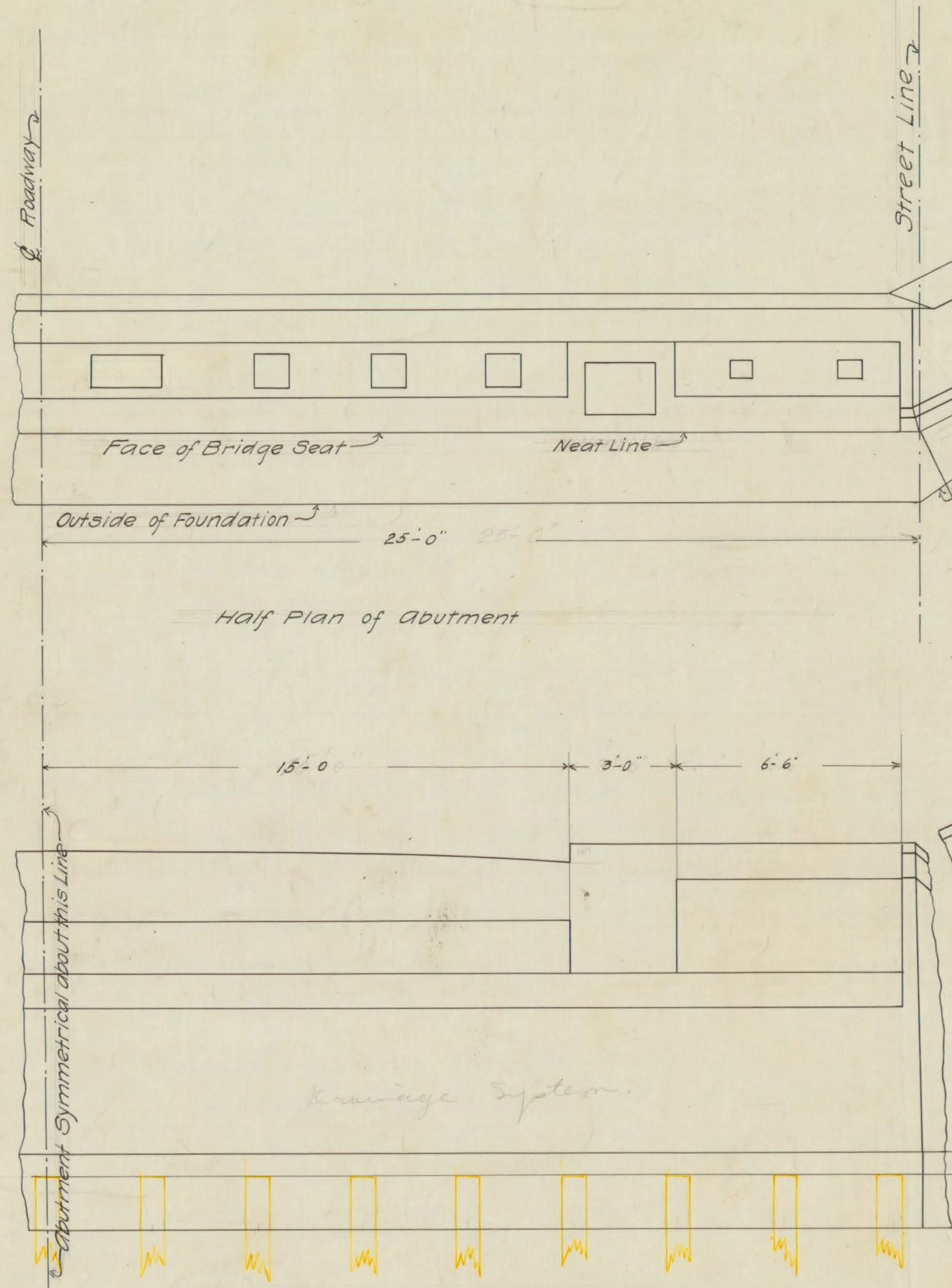
Half Elevation of Abutment Two Complete Abutments Required
