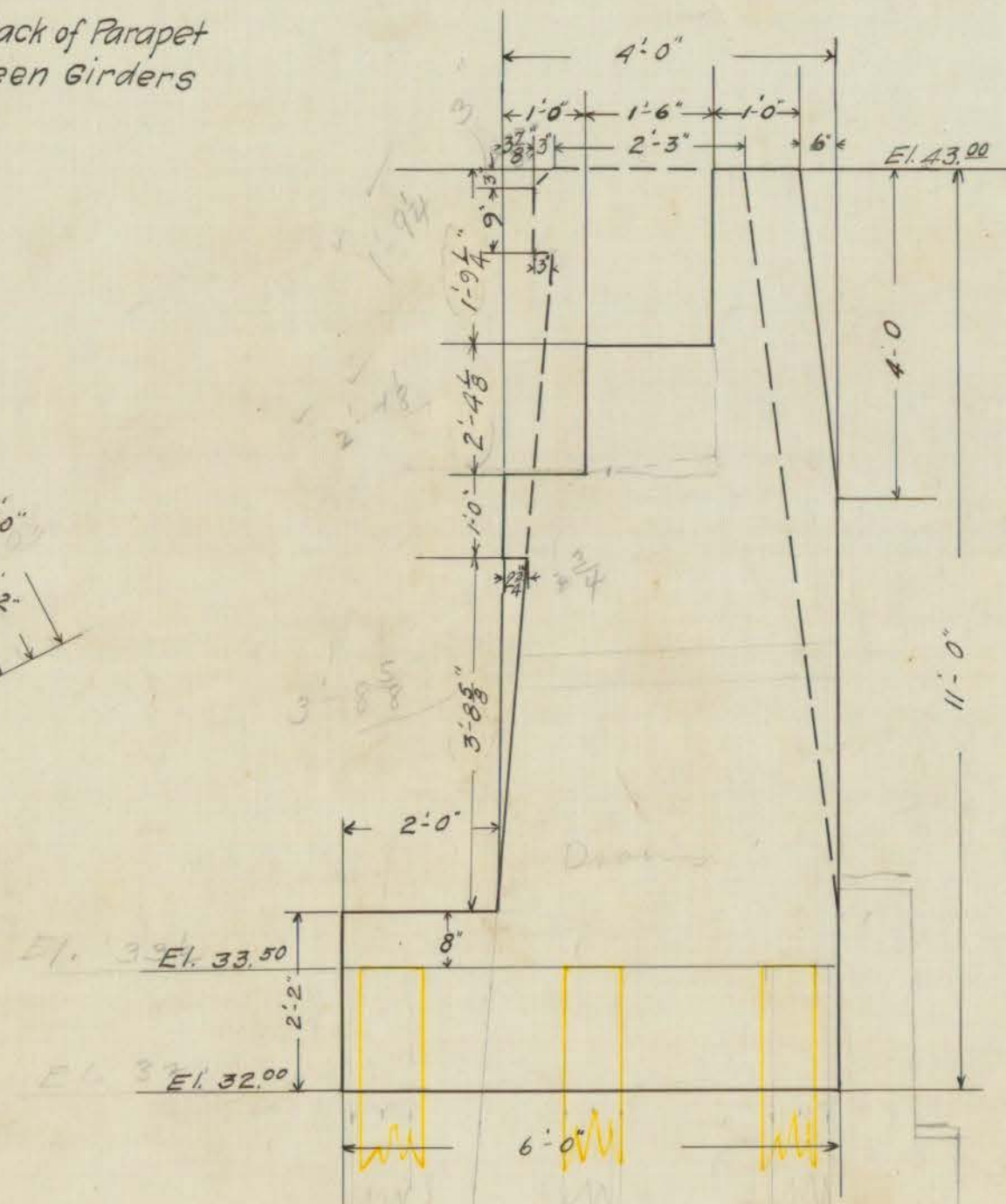
Section of Abutment on Center Line Broken Lines show Section of Wing Wall
