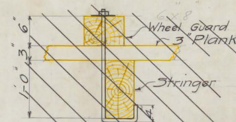
Detail at Wheel Guard
