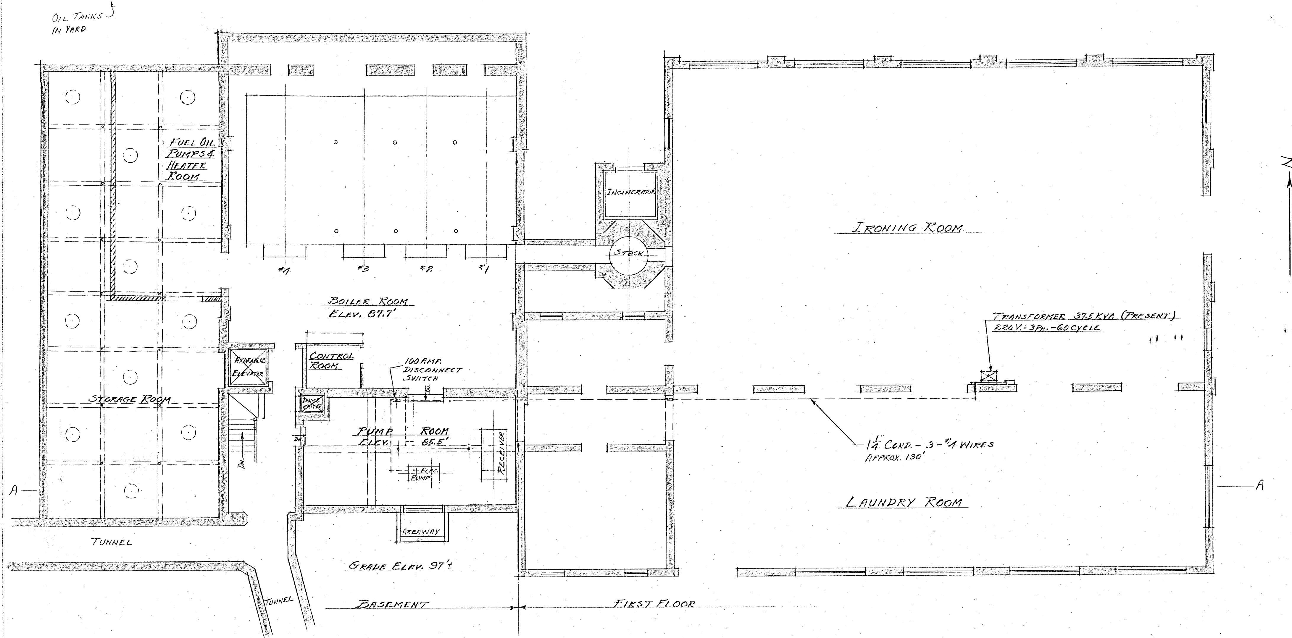
PLAN OF BOILER, PUMP AND LAUNDRY ROOMS SCALE - 1/8" = 1'-0"
