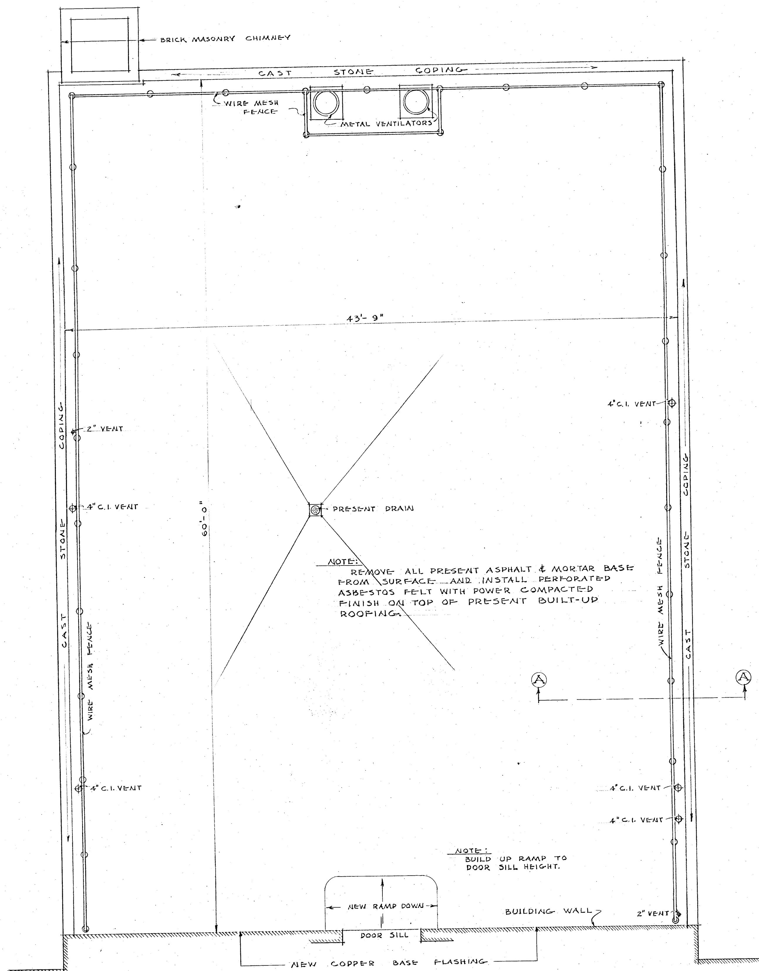
PLAN OF FOURTH FLOOR ROOF SCALE 1/4" = 1'-0"
