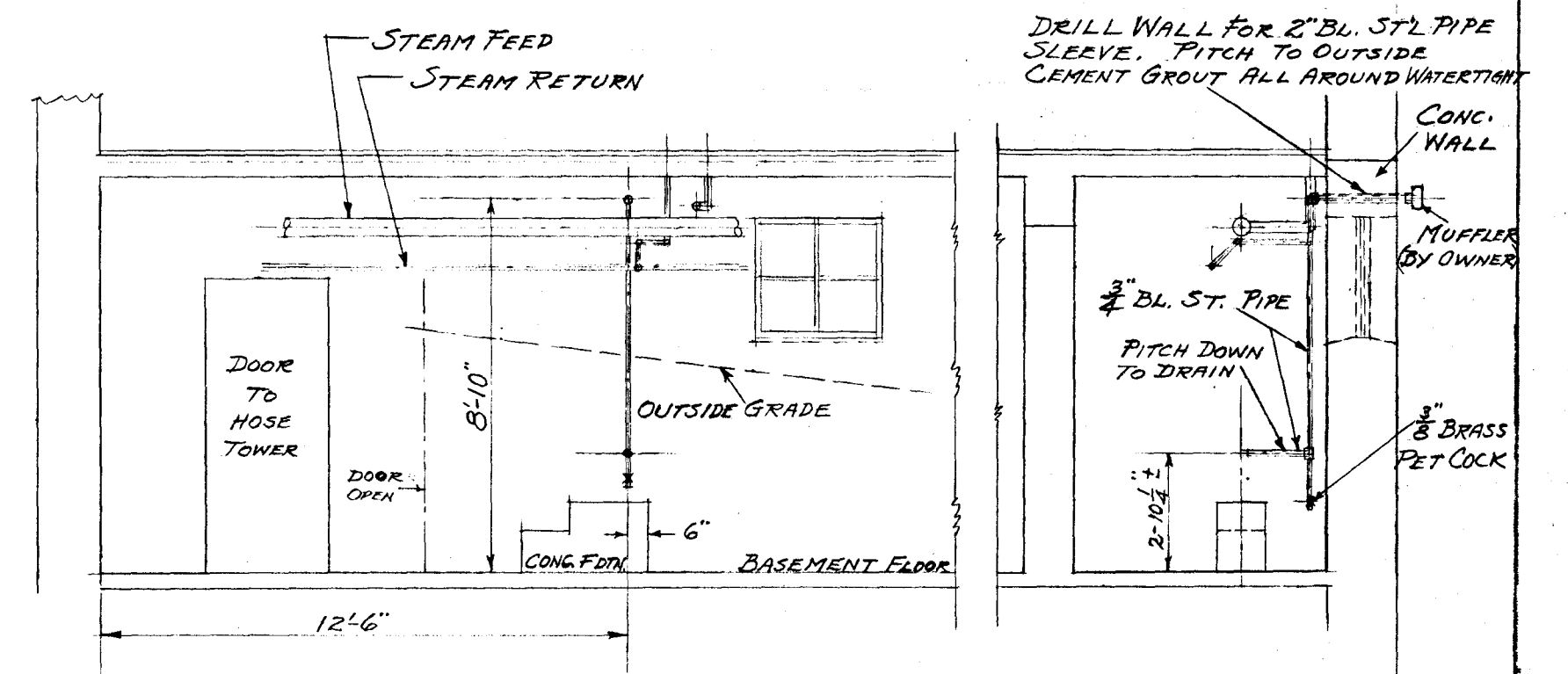
ELEV. LOOKING NORTH SCALE - 1/4" = 1'-0"
