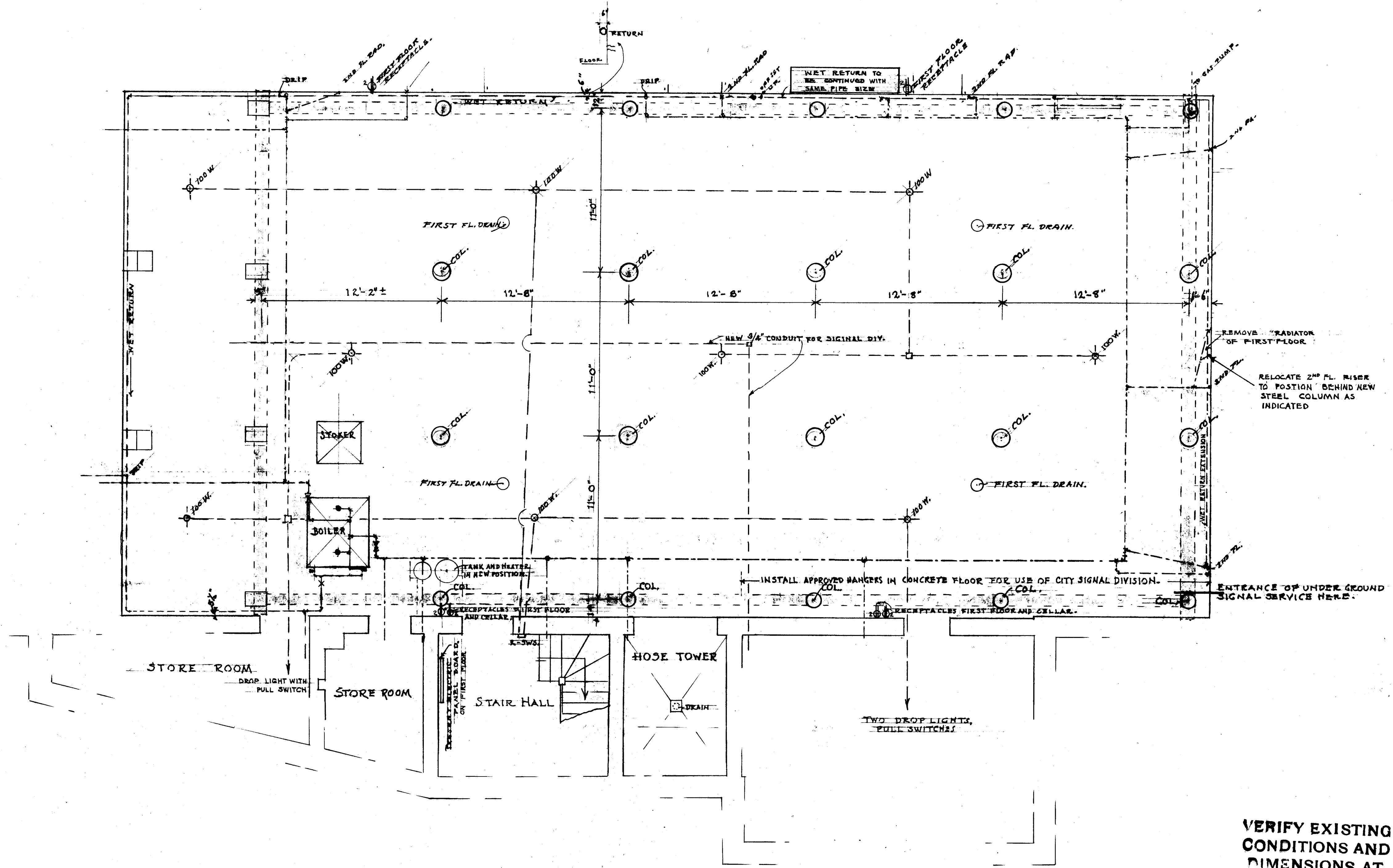
ELECTRICAL AND HEATING PLAN SCALE 1/4" = 1 FT.
