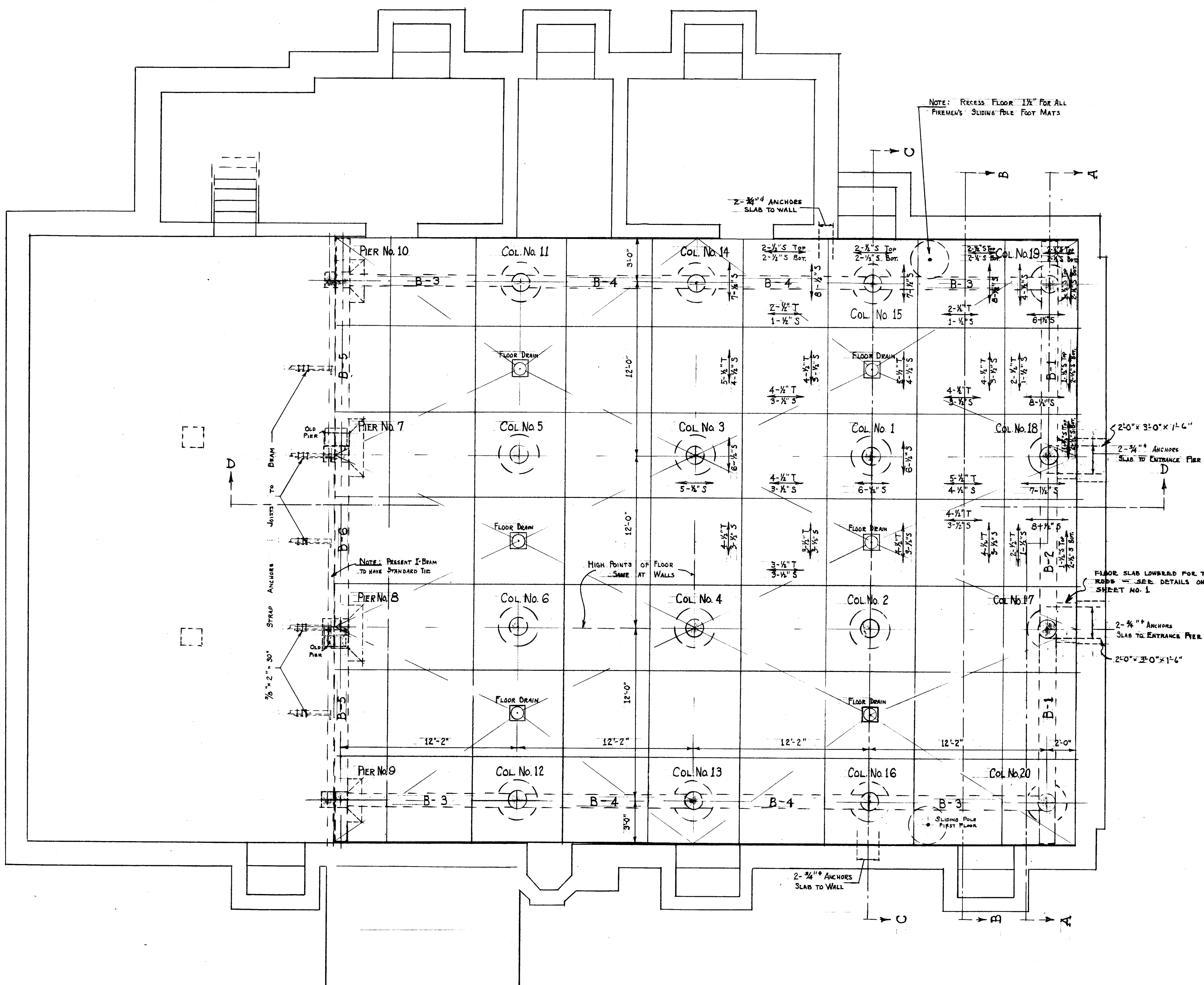
FIRST FLOOR FRAMING PLAN SCALE 1/4 IN. = 1 FT.
