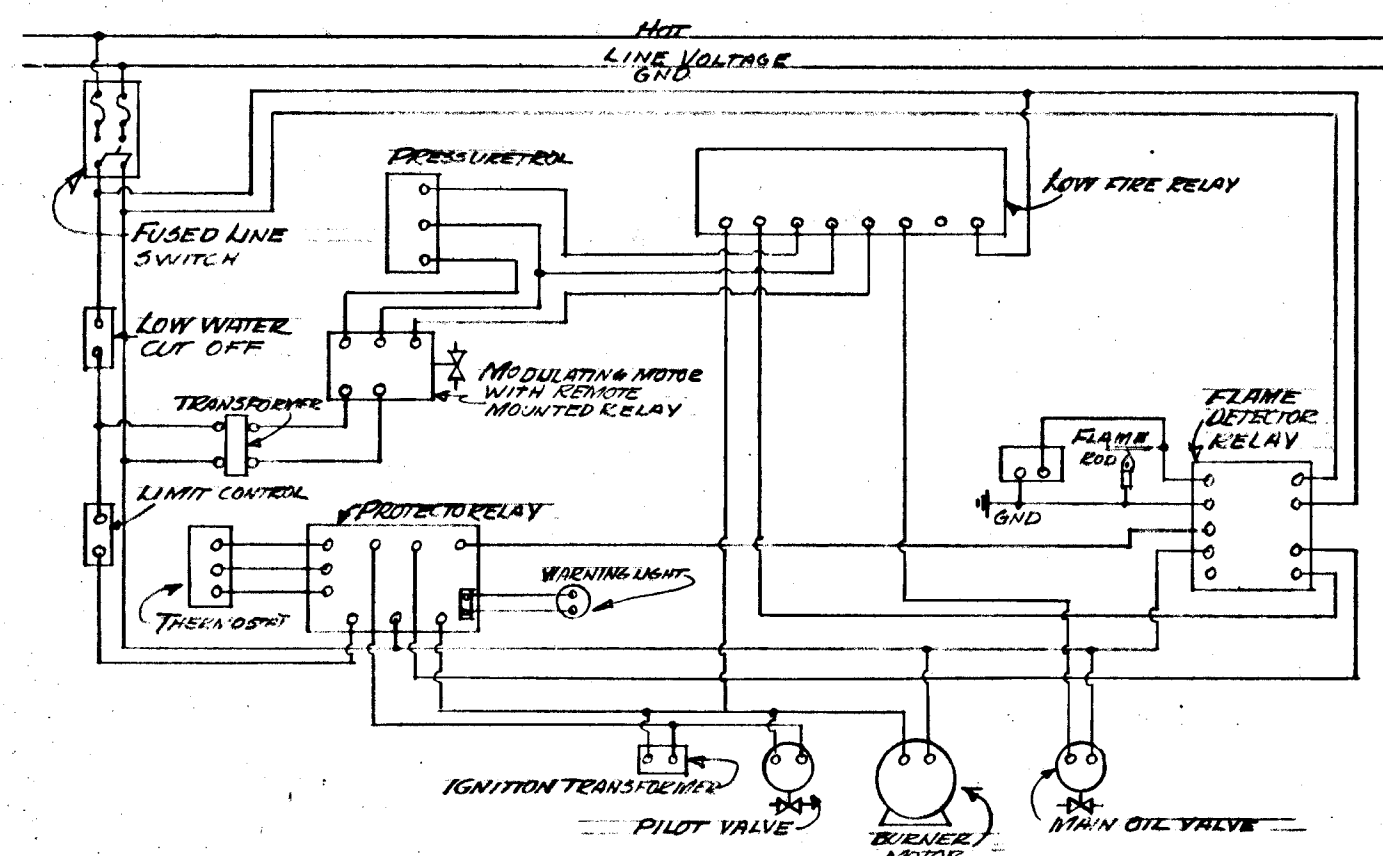
Schematic Control Diagram FOR EACH BURNER NO SCALE
