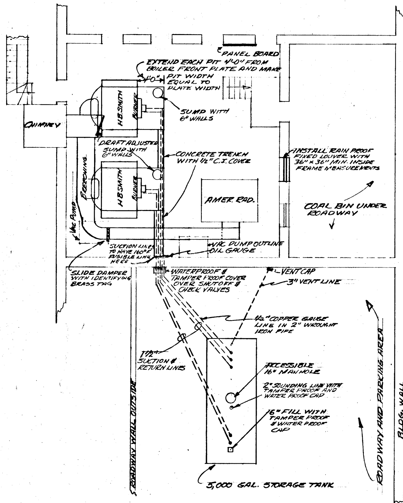
Boiler Room & Surrounding Area Plan Scale: 1/8" = 1'-0"
