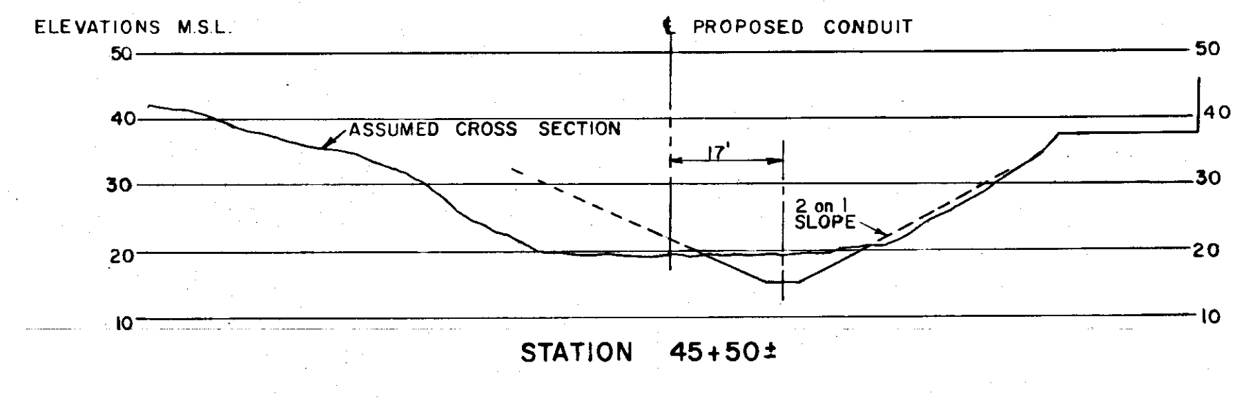
SECTIONS SECTIONS FACING UP-STREAM SCALE - HOR 1" = 20' VERT 1" = 20'
