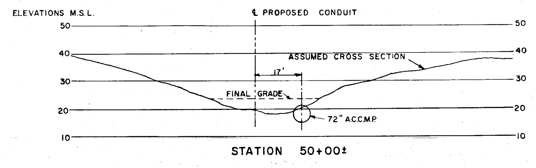
SECTIONS SECTIONS FACING UP-STREAM SCALE - HOR 1" = 20' VERT 1" = 20'
