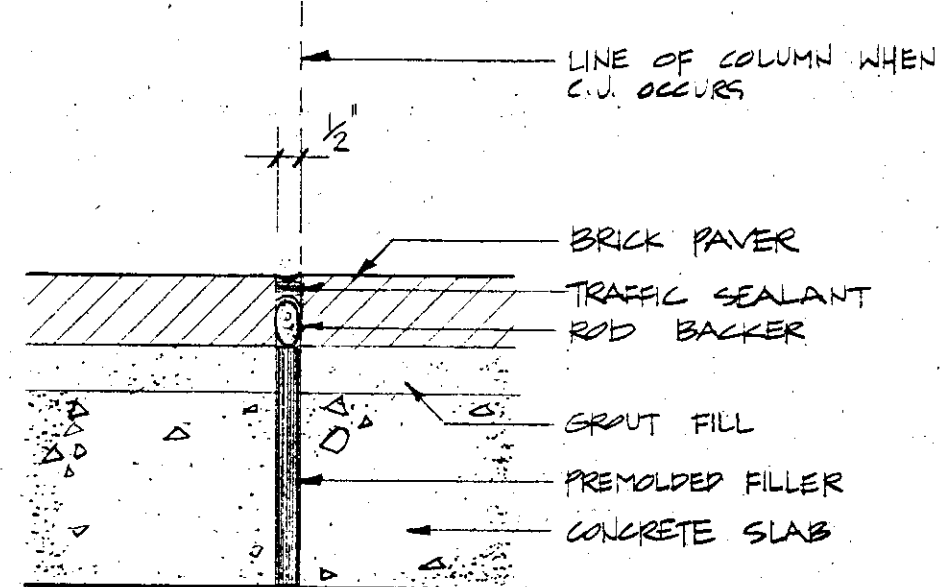
1 CONTROL JOINT SCALE: 3" = 1'-0"
