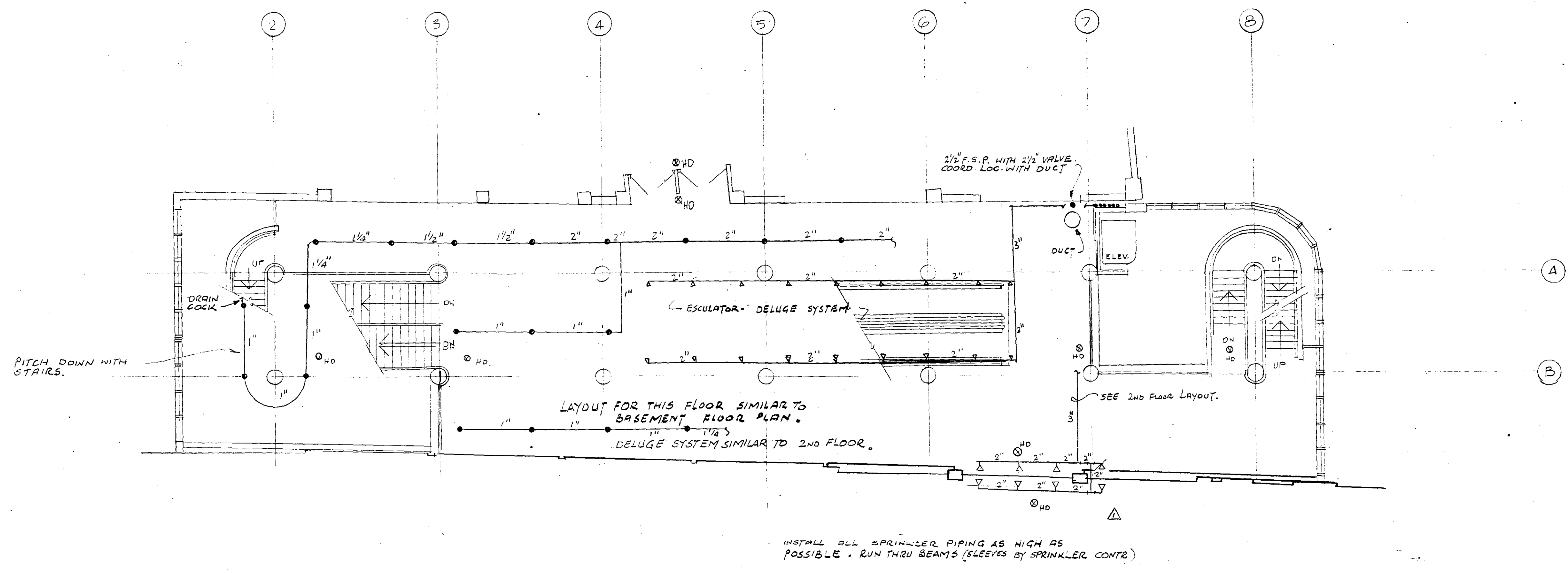
FIRST FLOOR PLAN (CEL 73.285) SCALE: 1/8" = 1'-0"
