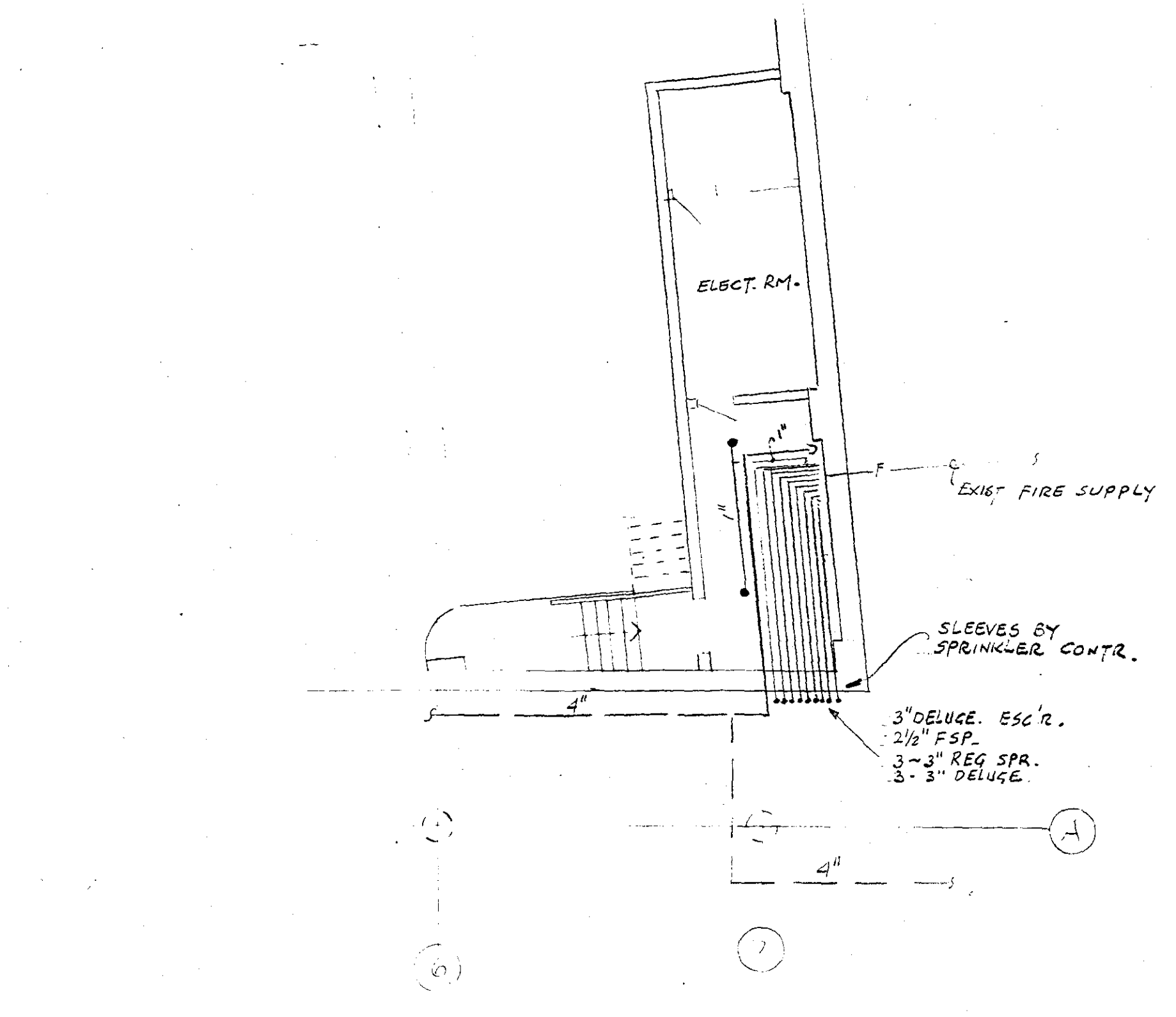
SUB-BASEMENT FLOOR PLAN (CEL 47.140) SCALE: 1/8" = 1'-0"
