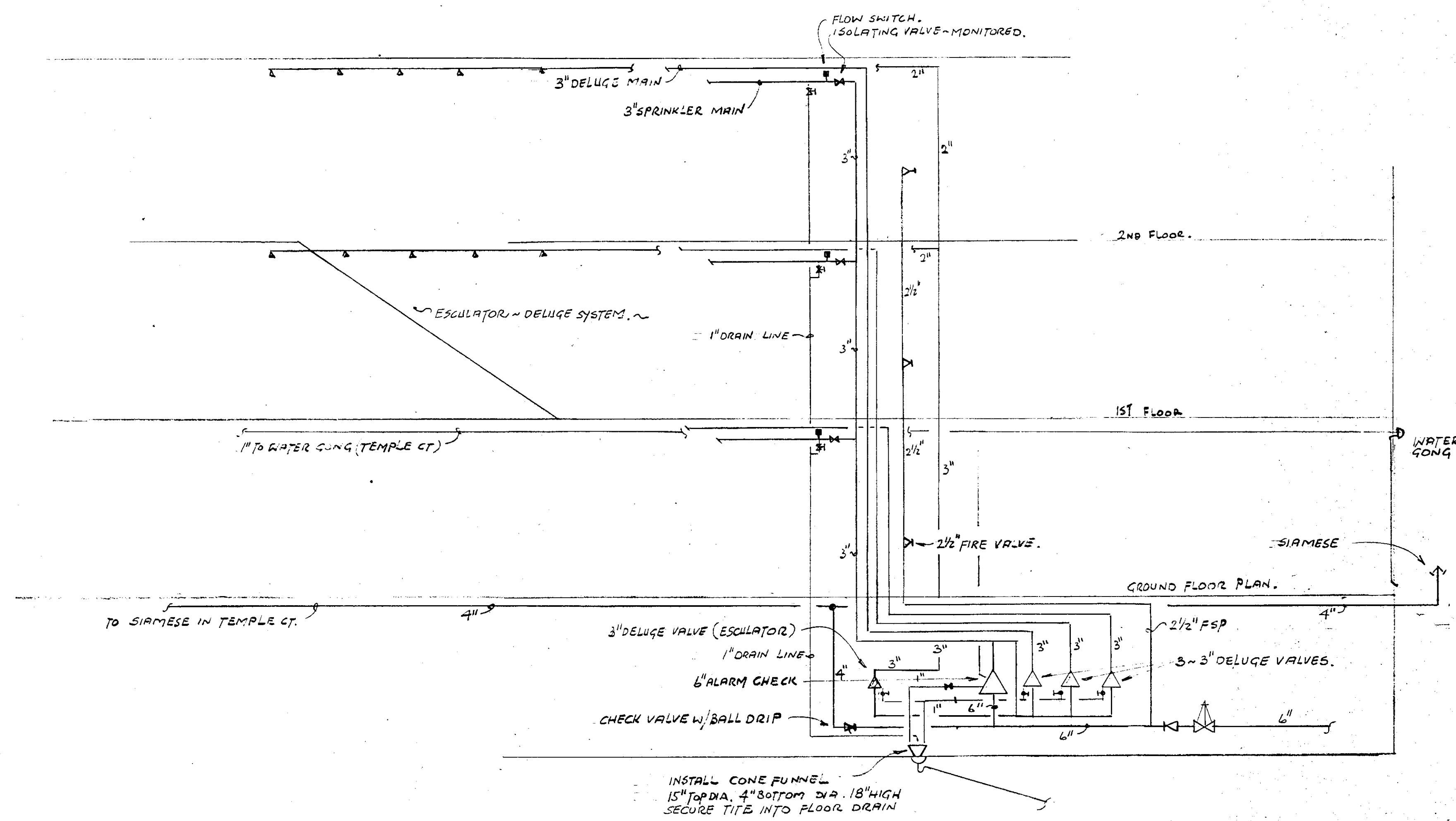
SPRINKLER & STANDPIPE RISER DIAGRAM.
