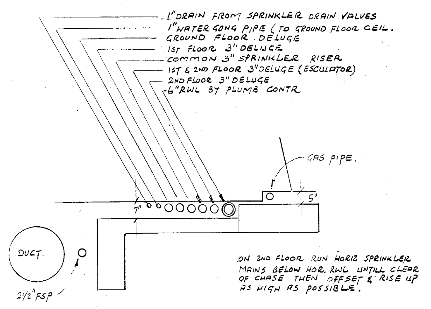
DETAIL OF CHASE SPACE. SCALE 3/8" = 1'-0"
