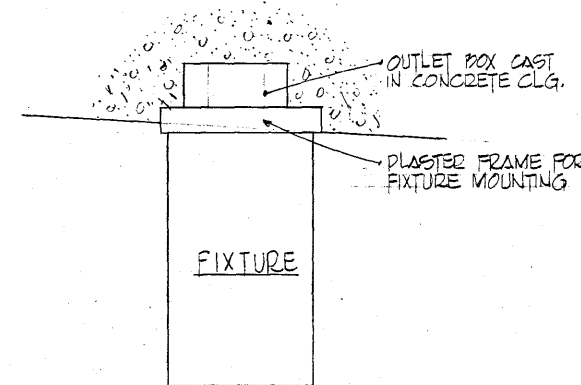
FIXTURE MOUNTING DETAIL N.T.S.
