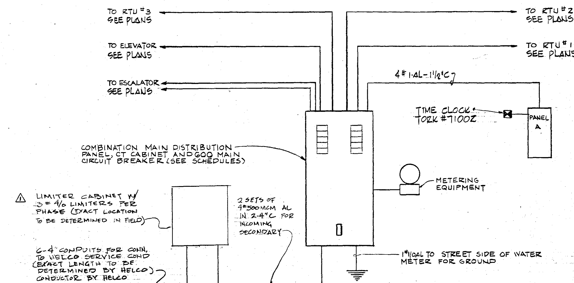
MAIN DISTRIBUTION RISER
