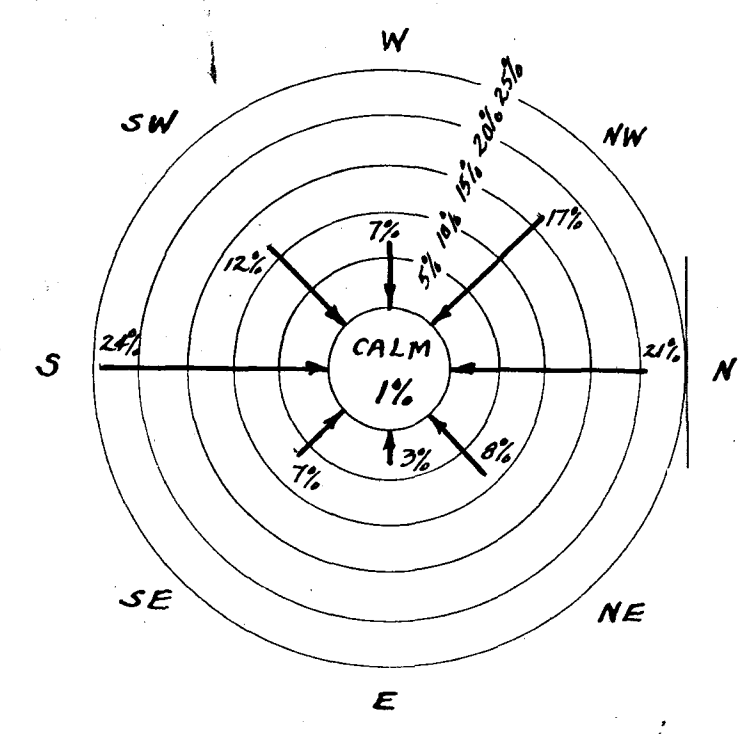
WIND ROSE Hartford, Connecticut
