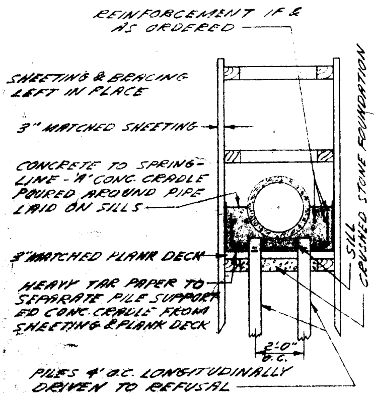
SPECIAL CONCRETE SEWER FOUNDATION WITH PILES
