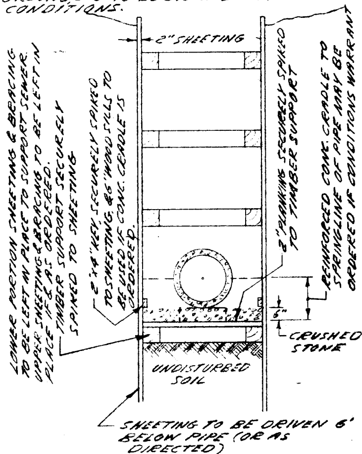
SPECIAL SEWER FOUNDATION FOR INADEQUATE SOIL CONDITIONS
