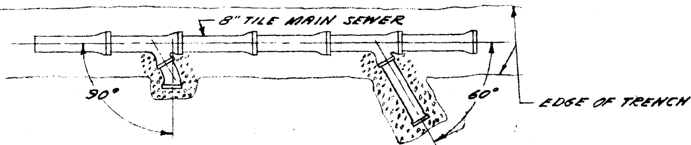
TYPICAL WYE BRANCH FOR TILE SEWER
