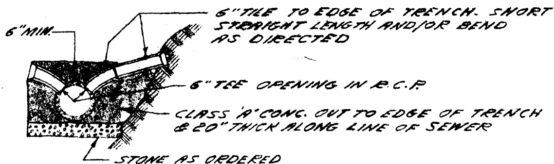
TYPICAL 6" BRANCH FOR R.C.P. SEWER
