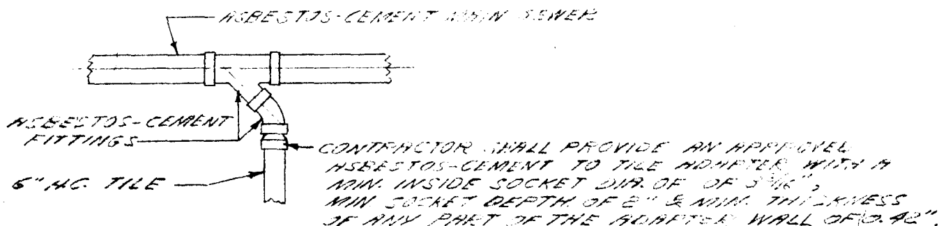
TYPICAL WYE BRANCH FOR ASBESTOS-CEMENT PIPE SEWER
