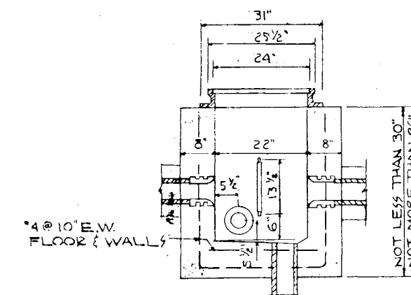
SECTION "F-F" TELEPHONE HANDHOLE
