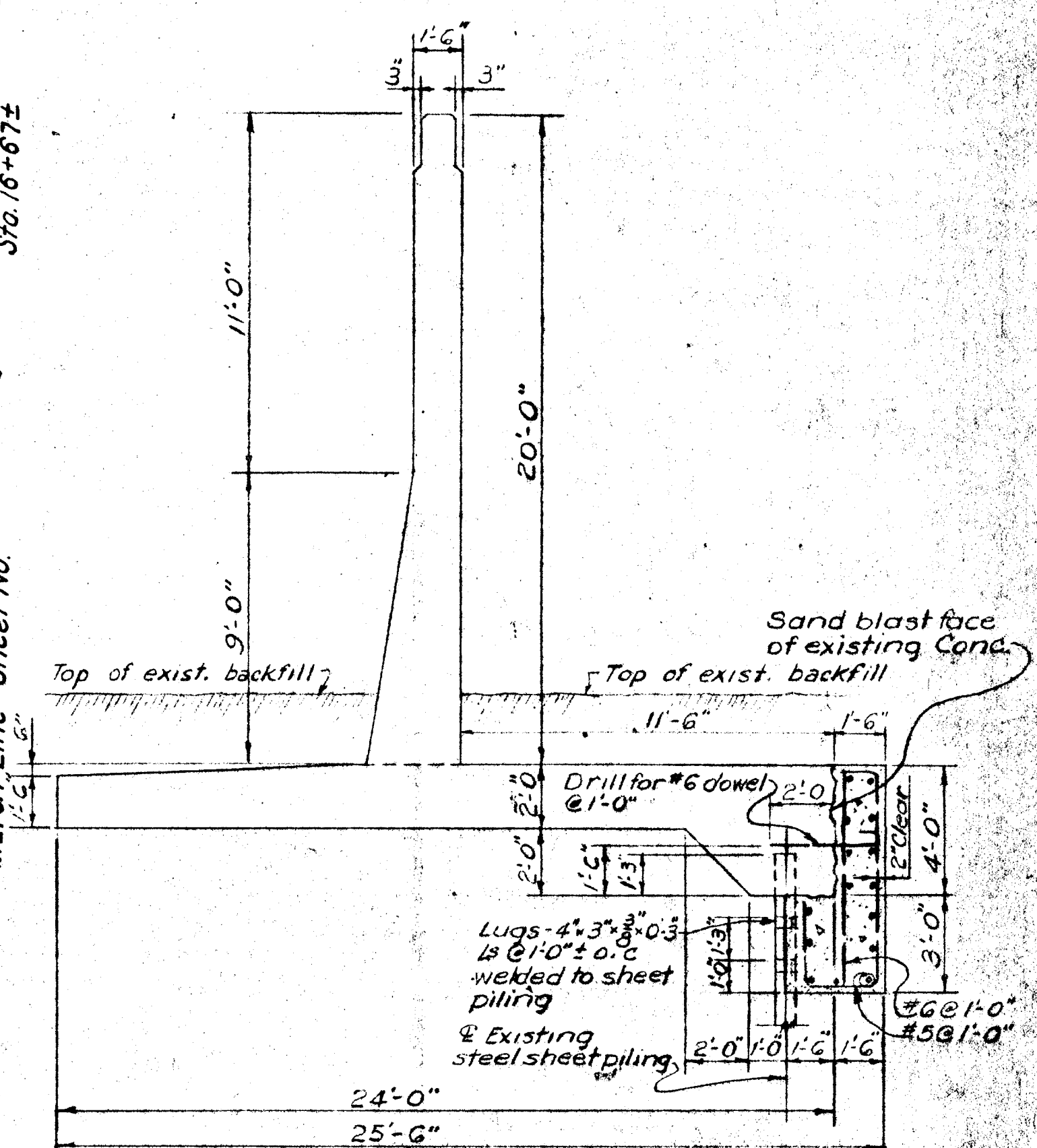
WALL MODIFICATION TYPE "D" SCALE: 1"=1'-0"
