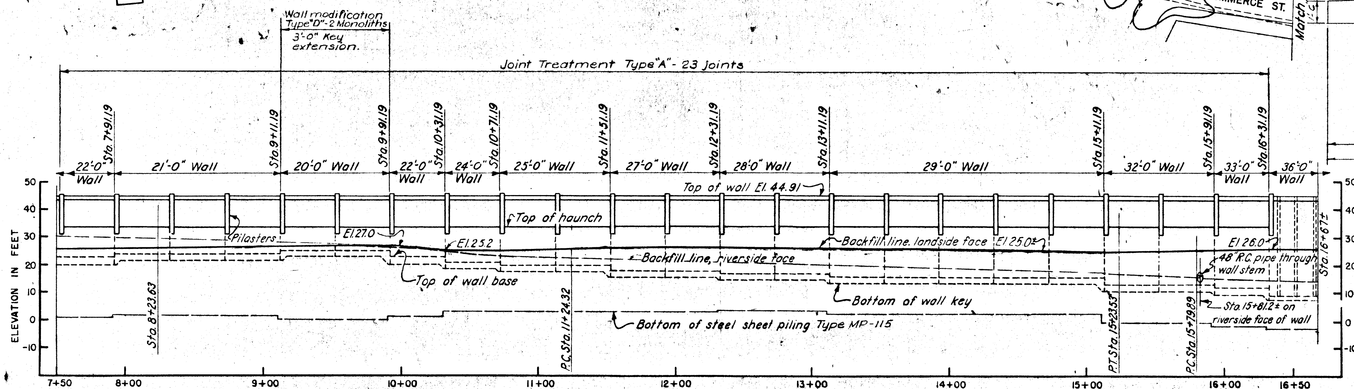
PROFILE SCALE: VERT. 1"=20'-0" HOR. 1"=40'-0"
