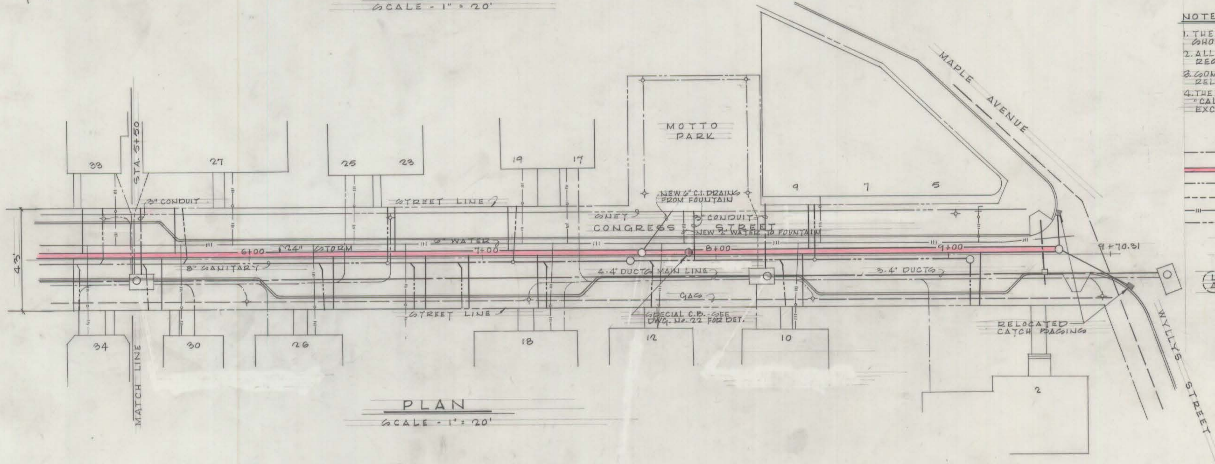
PLAN SCALE - 1" = 20'
