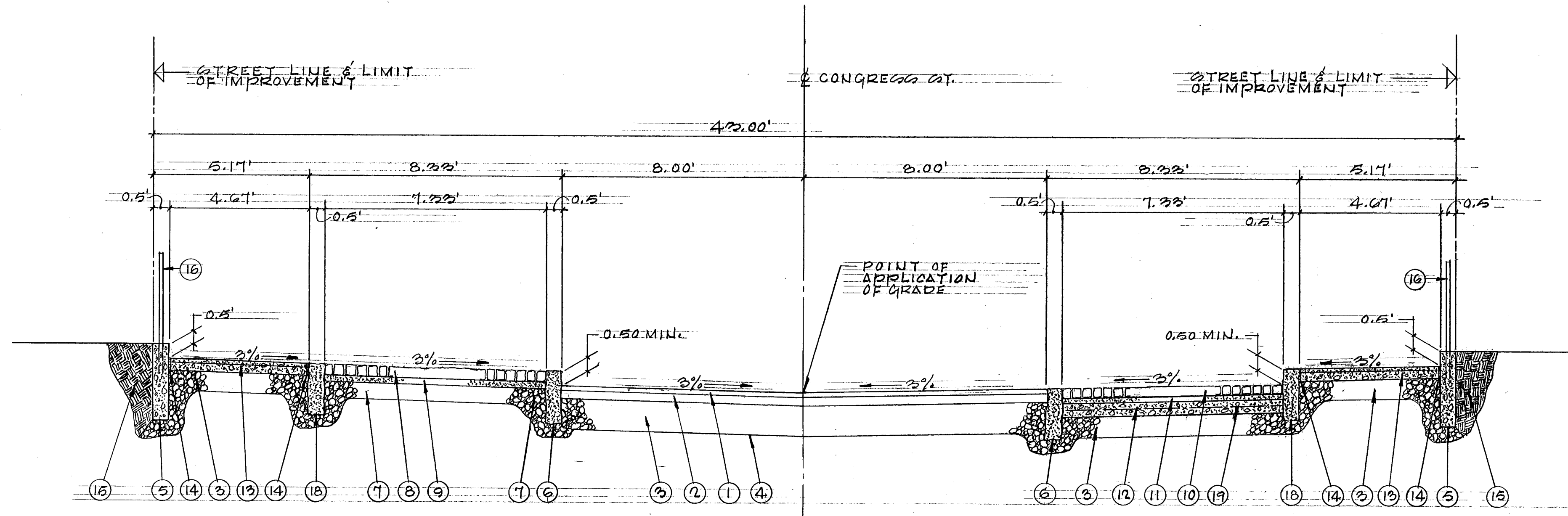
TYPICAL CROSS SECTION 2-2 CONGRESS STREET N.T.S.
