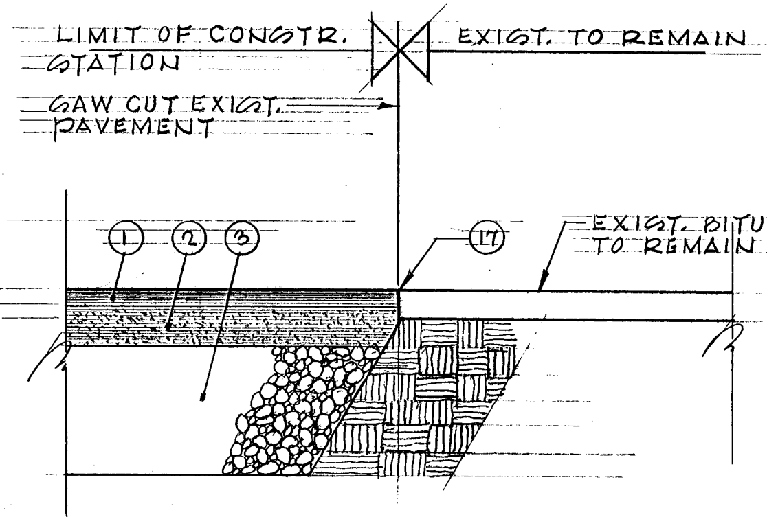
TRANSITION-NEW BITUM. PAV'T. TO EXIST. BITUM. PAV'T. CONGRESS STREET N.T.S.
