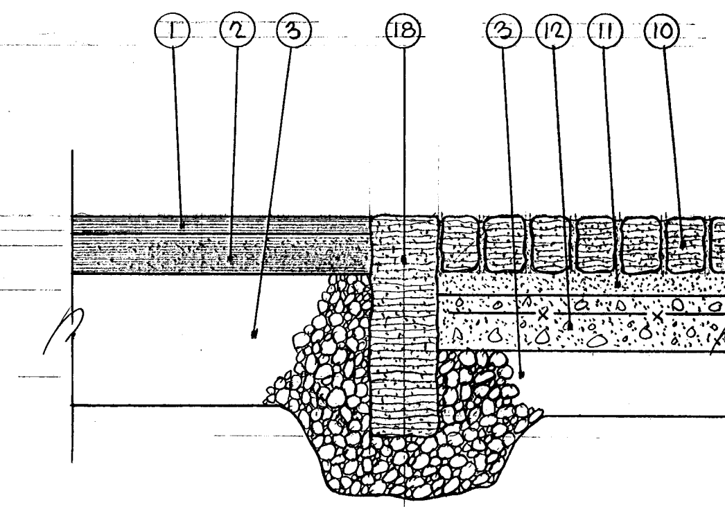
TRANSITION-BITUM. PAV'T TO COBBLE PAV'T. CONGRESS STREET N.T.S.
