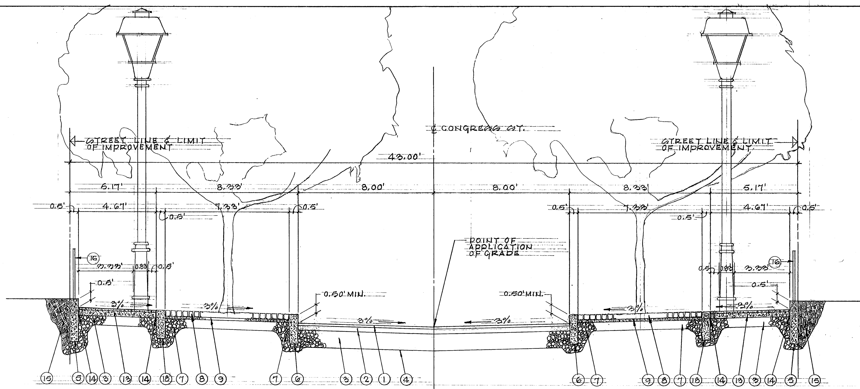
TYPICAL CROSS SECTION 1-1 CONGRESS STREET N.T.S.
