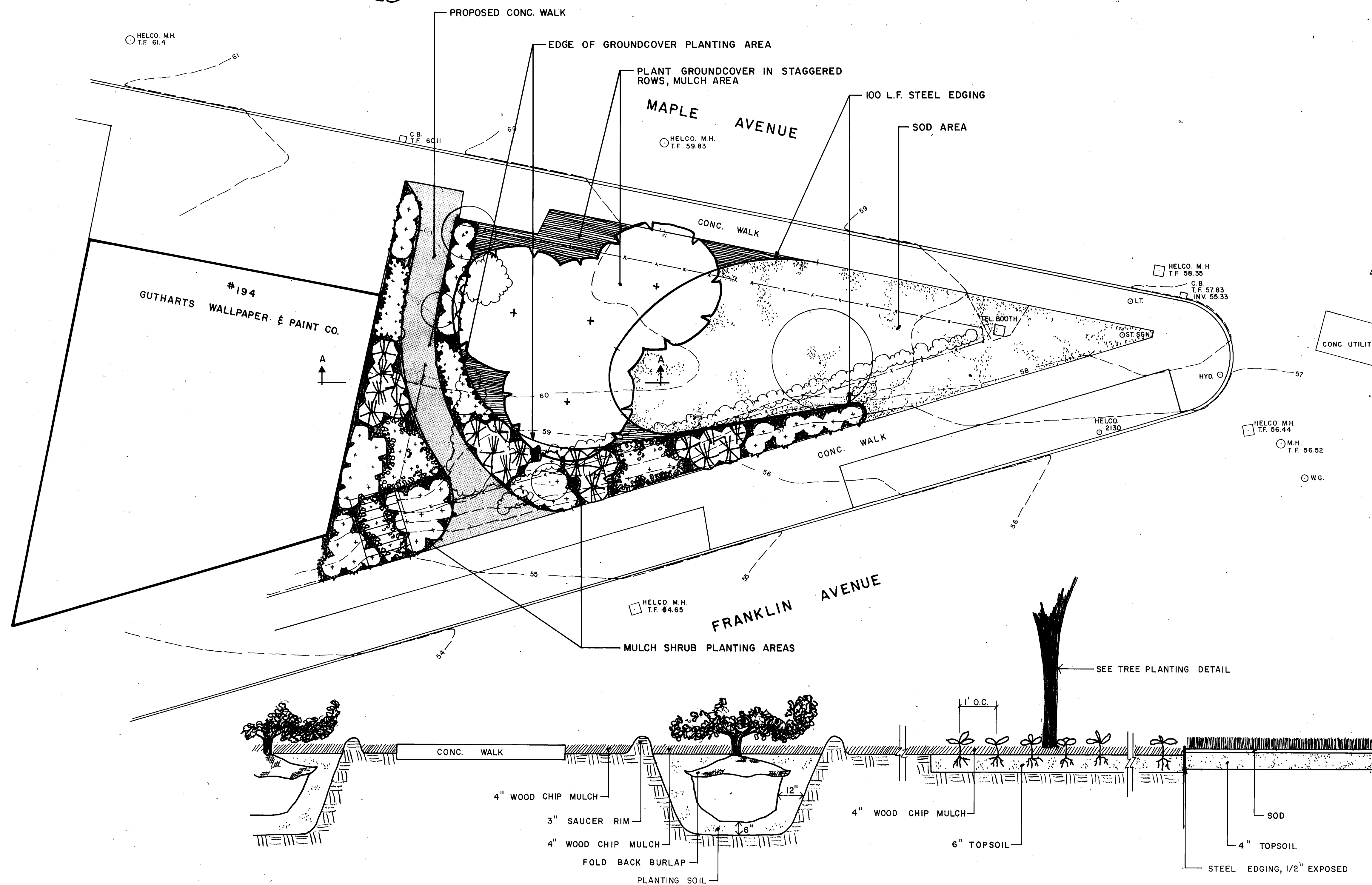
SHRUB & GROUNDCOVER PLANTING DETAILS SECTION A-A NO SCALE
