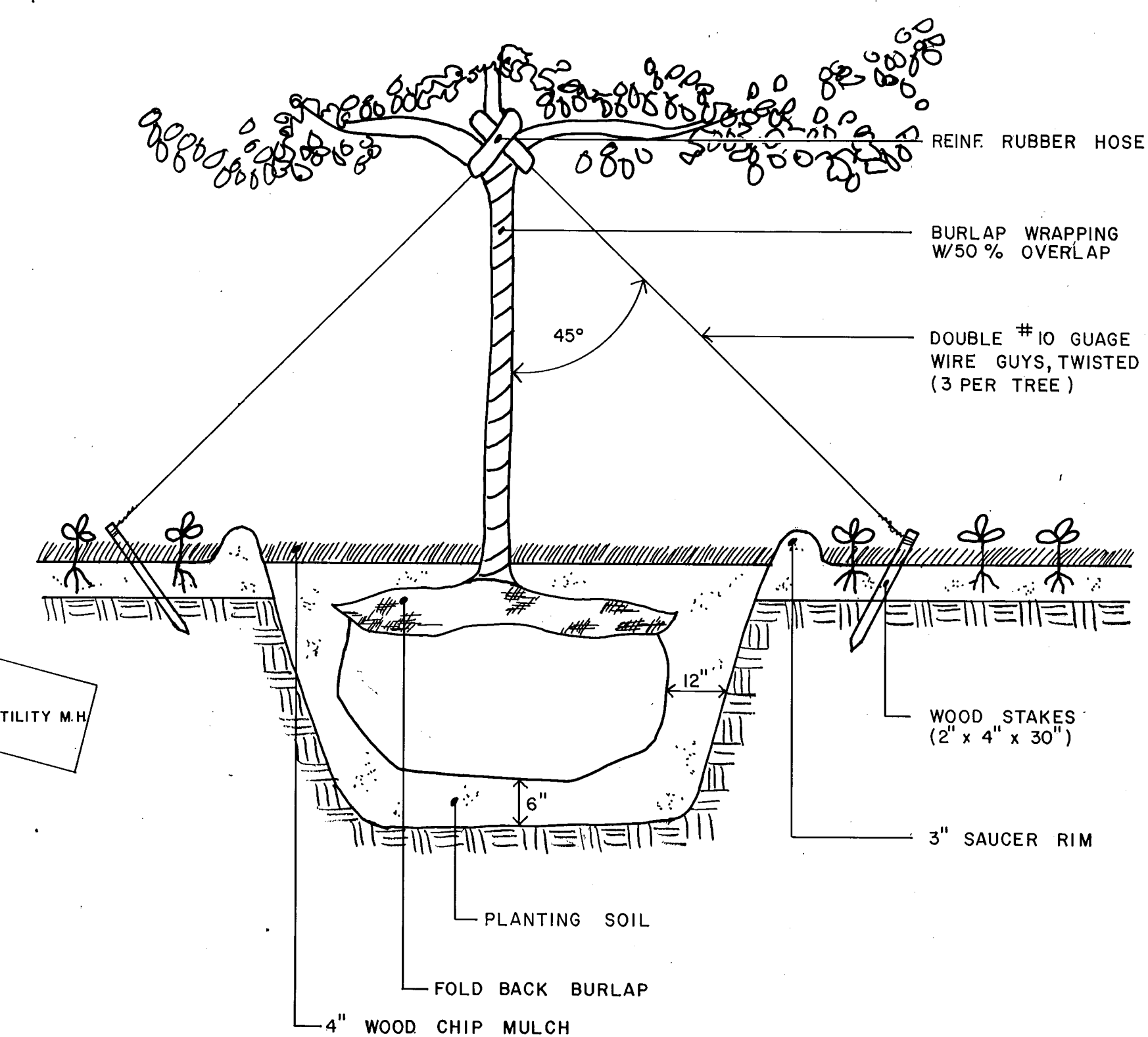
TREE PLANTING DETAIL NO SCALE
