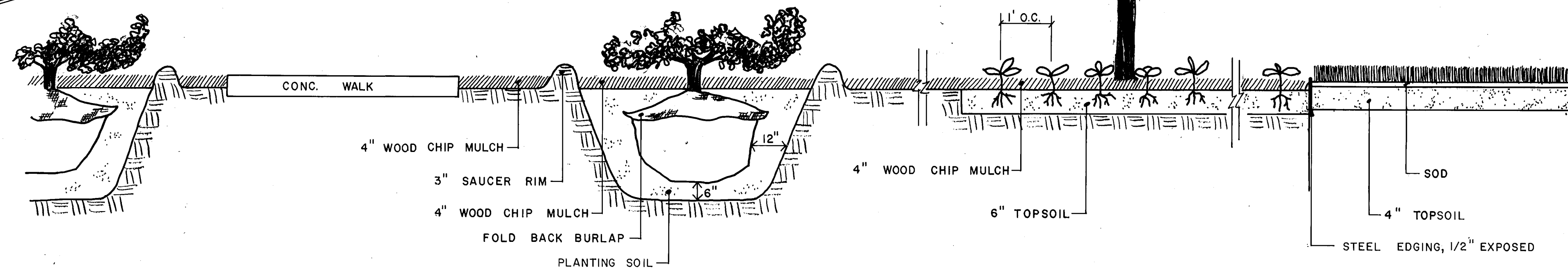
SHRUB & GROUNDCOVER PLANTING DETAILS SECTION A-A NO SCALE
