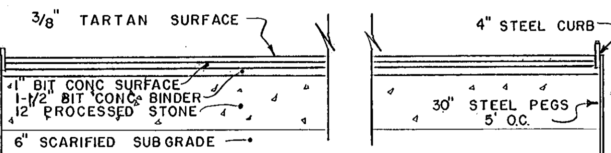
EXISTING TRACK PAVEMENT
