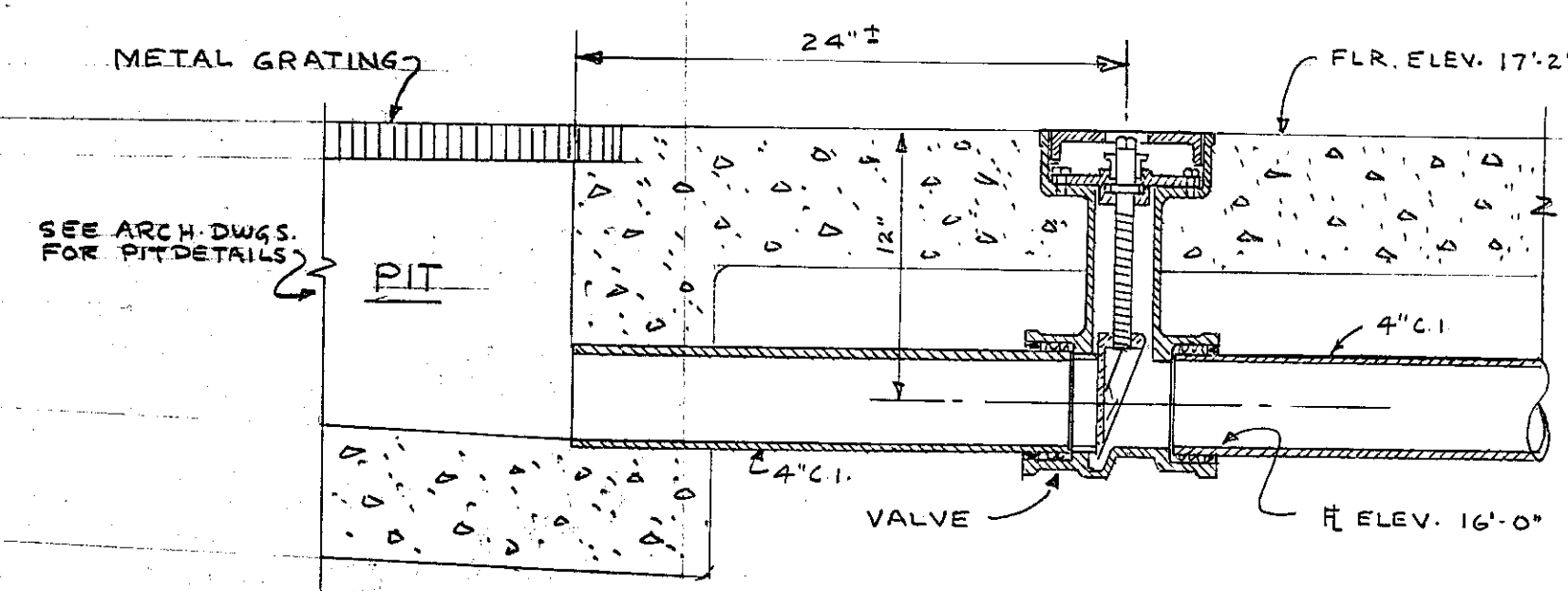
DETAIL VALVE AND PIT SCALE 1/2"=1'-0"
