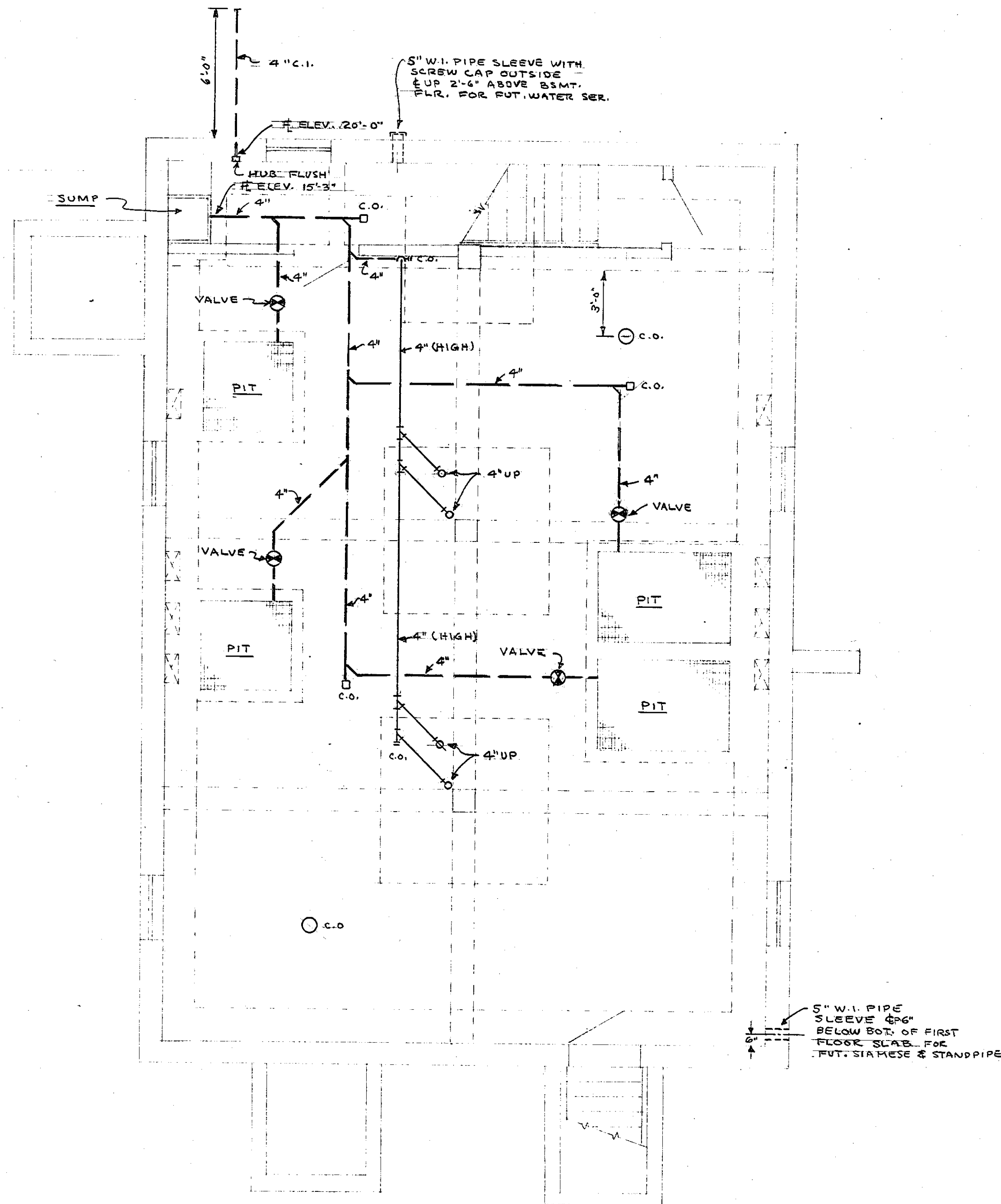
BASEMENT FLOOR PLAN SCALE 1/2"=1'-0"
