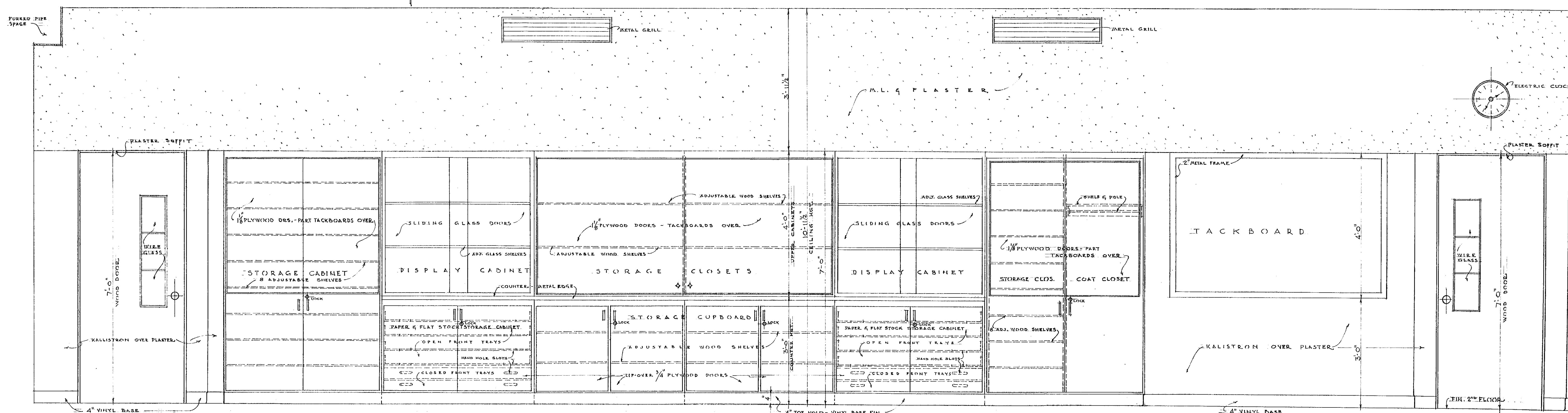
ELEVATION OF EAST WALL - ARTS & CRAFTS - SECOND FLOOR - Scale \frac{3}{4}" = 1'-0"
