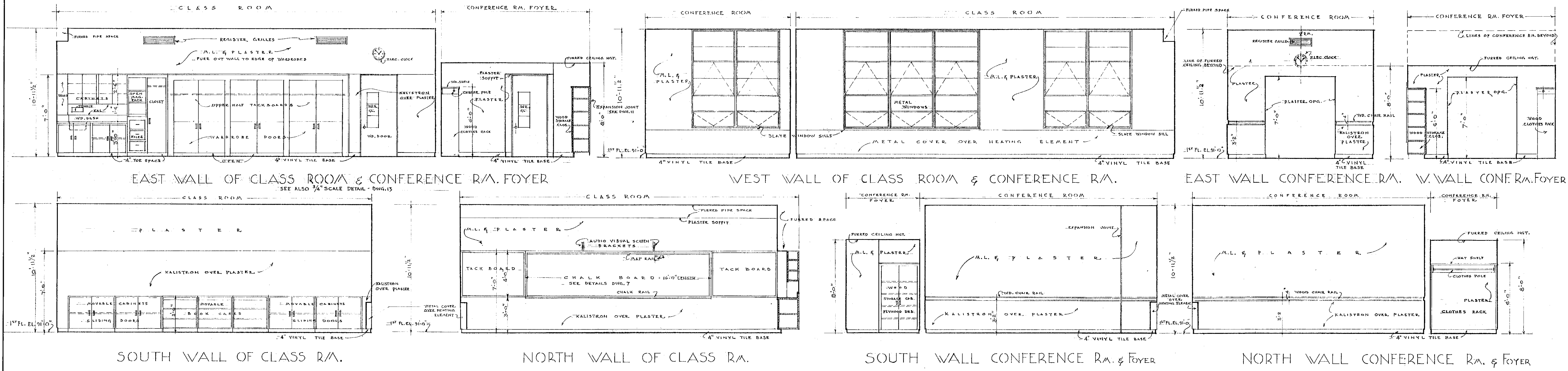
INTERIOR ELEVATIONS OF CLASS ROOM & CONFERENCE ROOM - 1 ST FLOOR SCALE 1/4"=1'-0"
