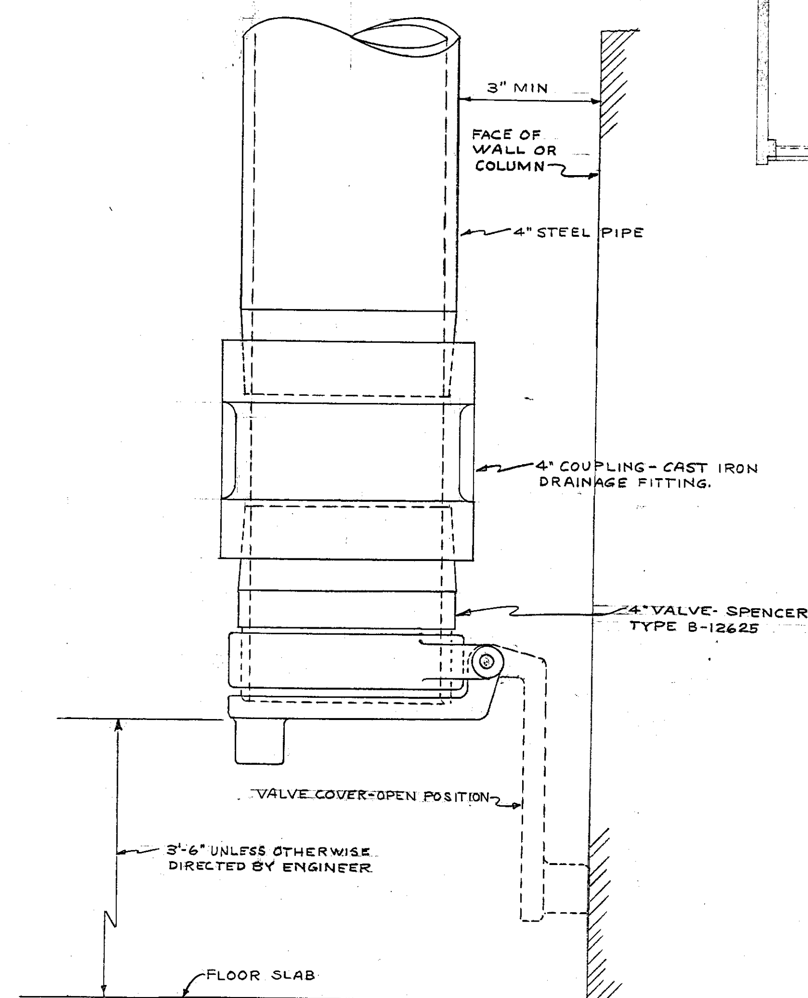
DETAIL- VALVE-HEAVY DUTY SYSTEM SCALE - 1/2" = 1"
