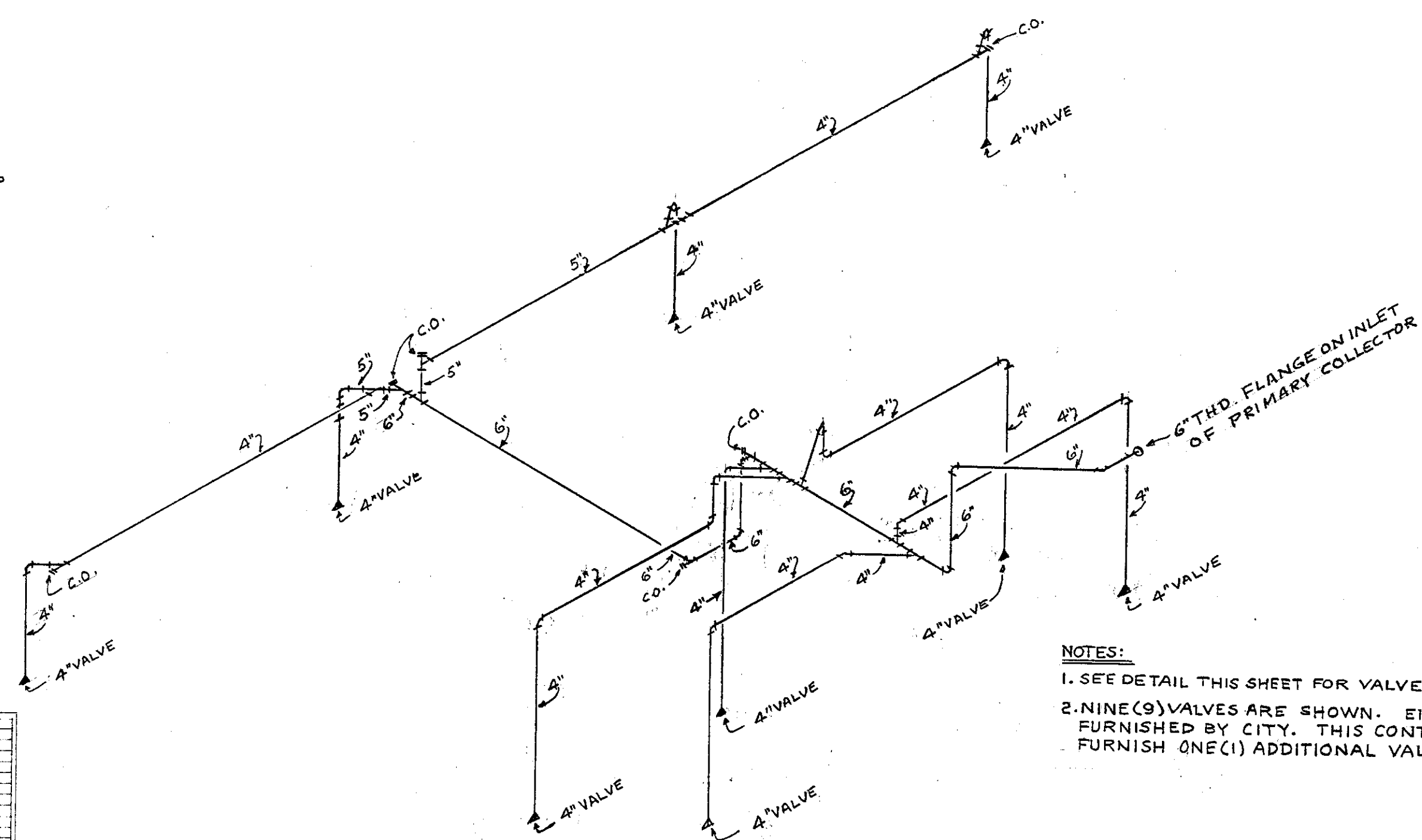
SCHEMATIC PIPING DIAGRAM-HEAVY DUTY VACUUM CLEANING SYSTEM NO SCALE
