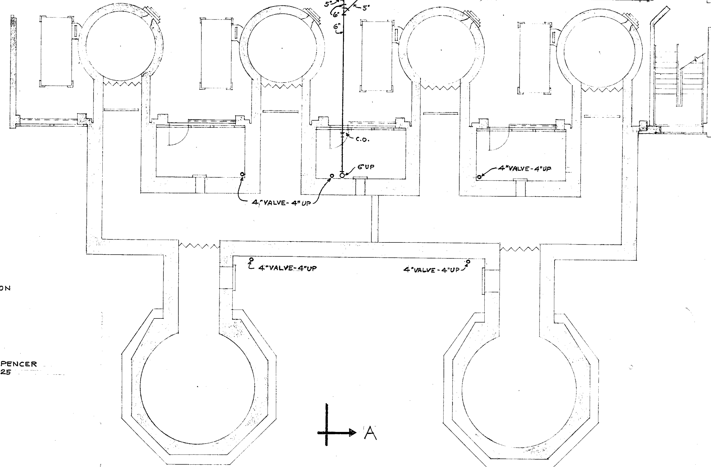
ASH TUNNEL FLOOR PLAN SCALE 1/8" = 1'-0"
