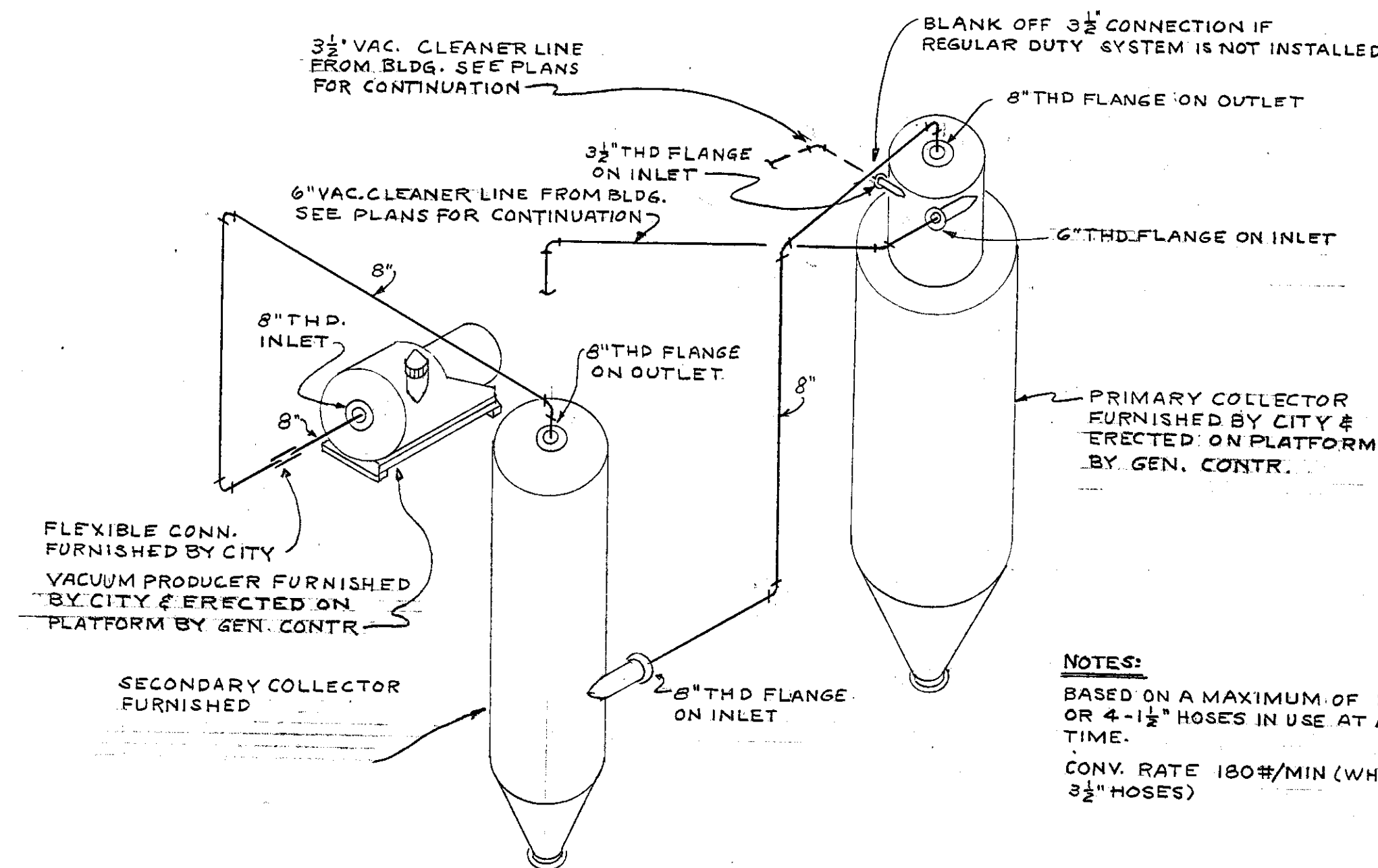
SCHEMATIC PIPING DIAGRAM-COLLECTORS NO SCALE
