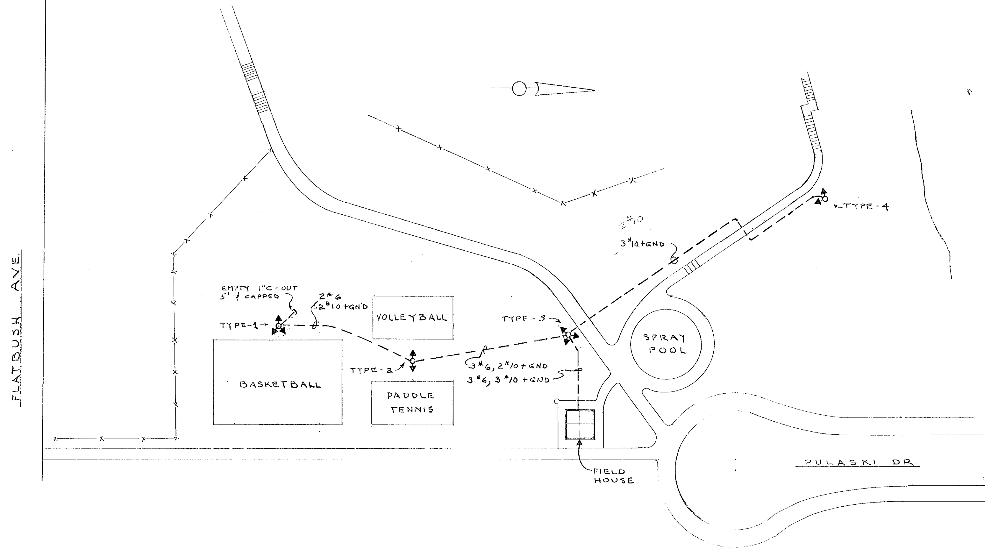
PLOT PLAN 1" = 40'
