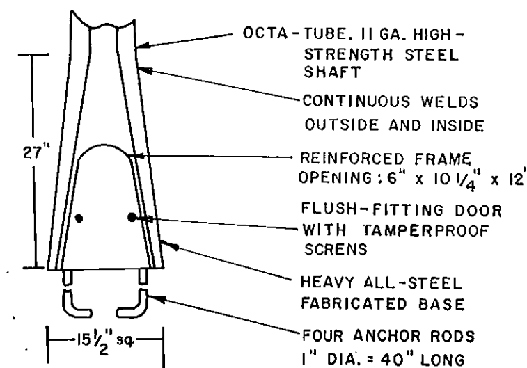
BASE DETAIL NO SCALE
