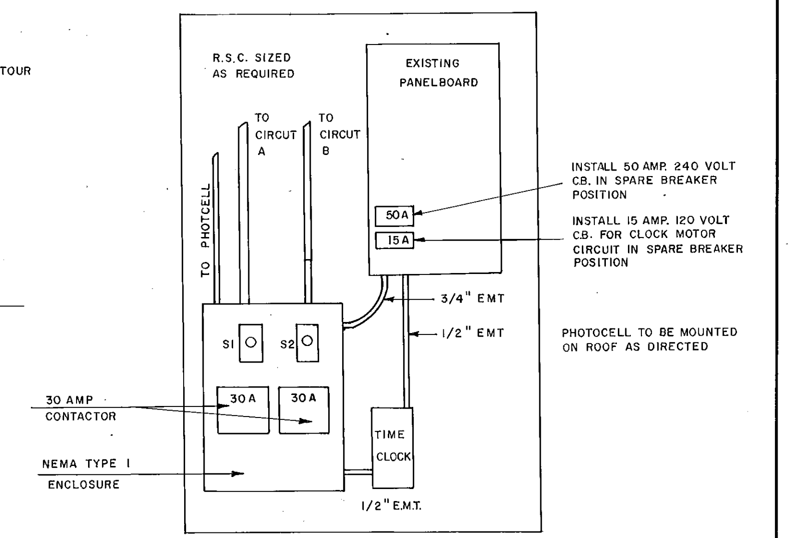
ELECTRICAL CONTROL SCHEMATIC DIAGRAM NOT TO SCALE
