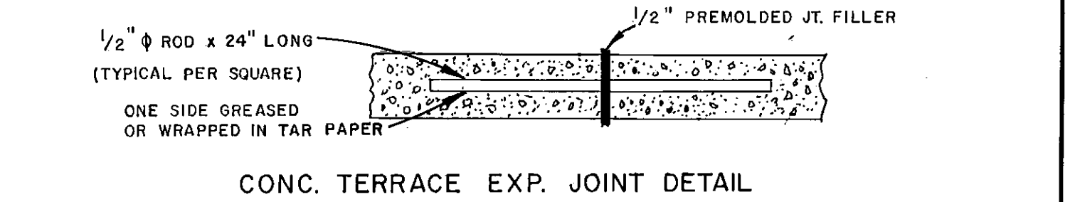
CONC. TERRACE EXP. JOINT DETAIL
