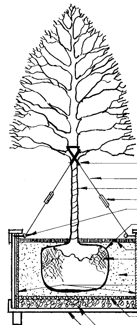
2 TREE PLANTING DETAIL 1/2\"/>
