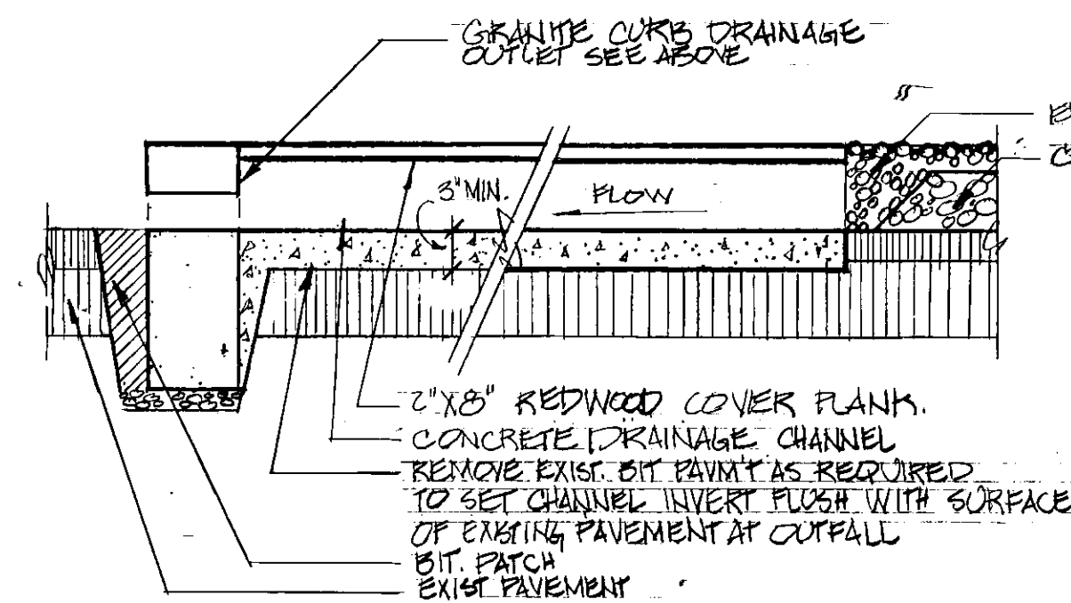
4 CONCRETE DRAINAGE CHANNEL WITH CURB DRAINAGE OUTLET NOT TO SCALE
