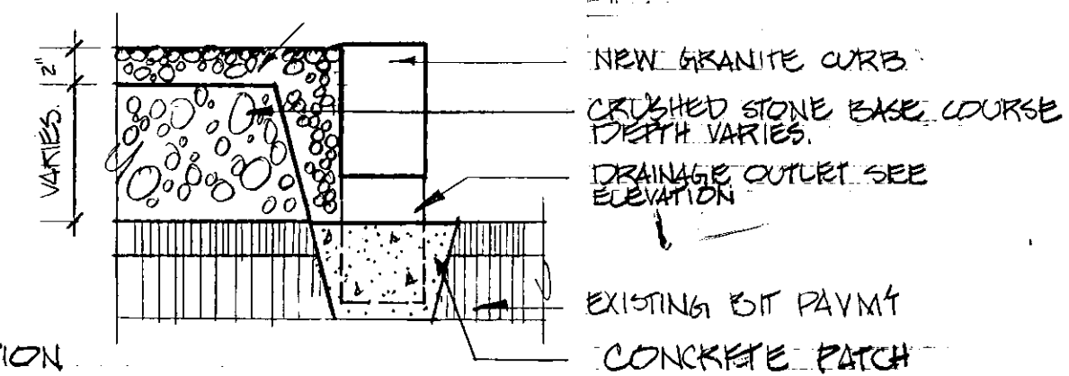
3 CURB DRAINAGE OUTLET 1\"/>
