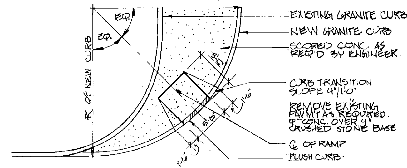
1 DROP CURB AND RAMP FOR HANDICAPPED 1/8" = 1'-0"
