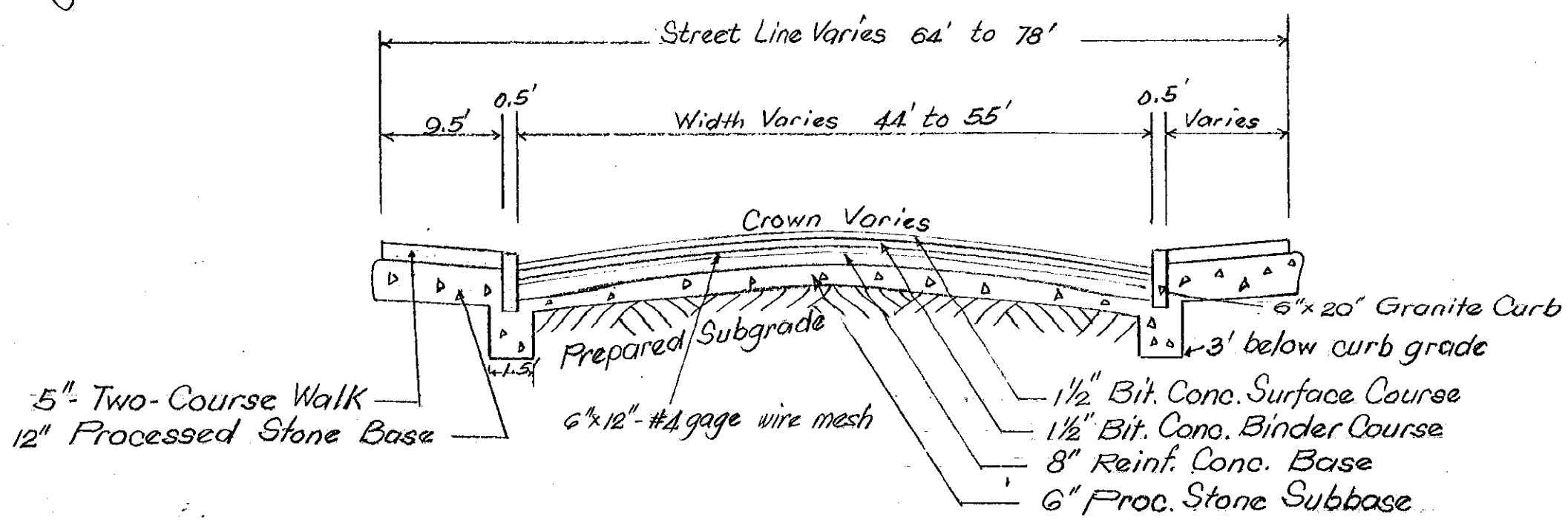
TYPICAL CROSS SECTION SCALE: Hor: 1"=10' Ver: 1"=4' FROM STA 2100 TO STA 7150
