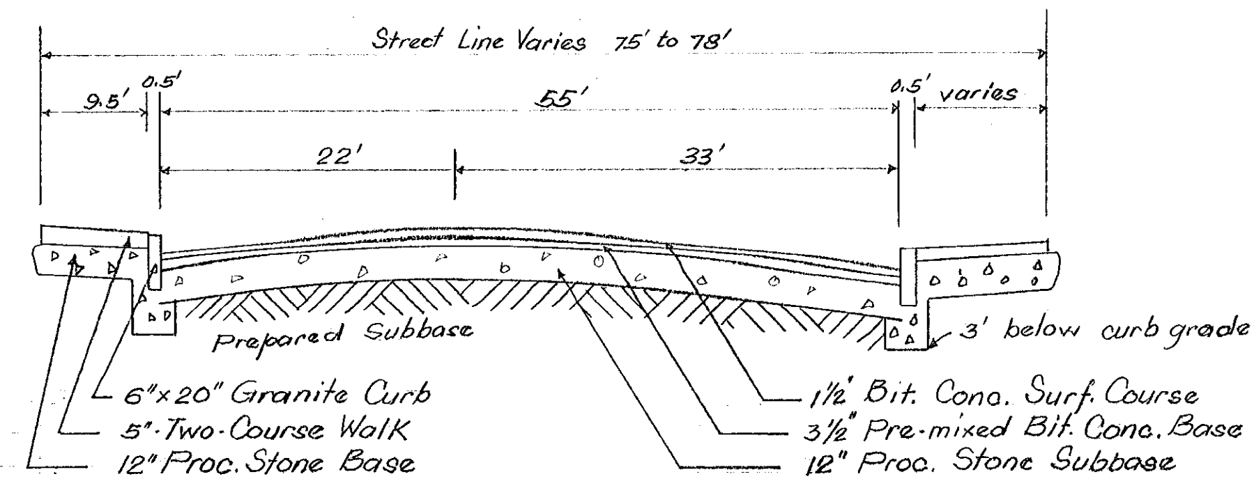
TYPICAL CROSS-SECTION SCALE: Hor: 1"=10' Ver: 1"=4' FROM STA 0+00 TO STA 2+00
