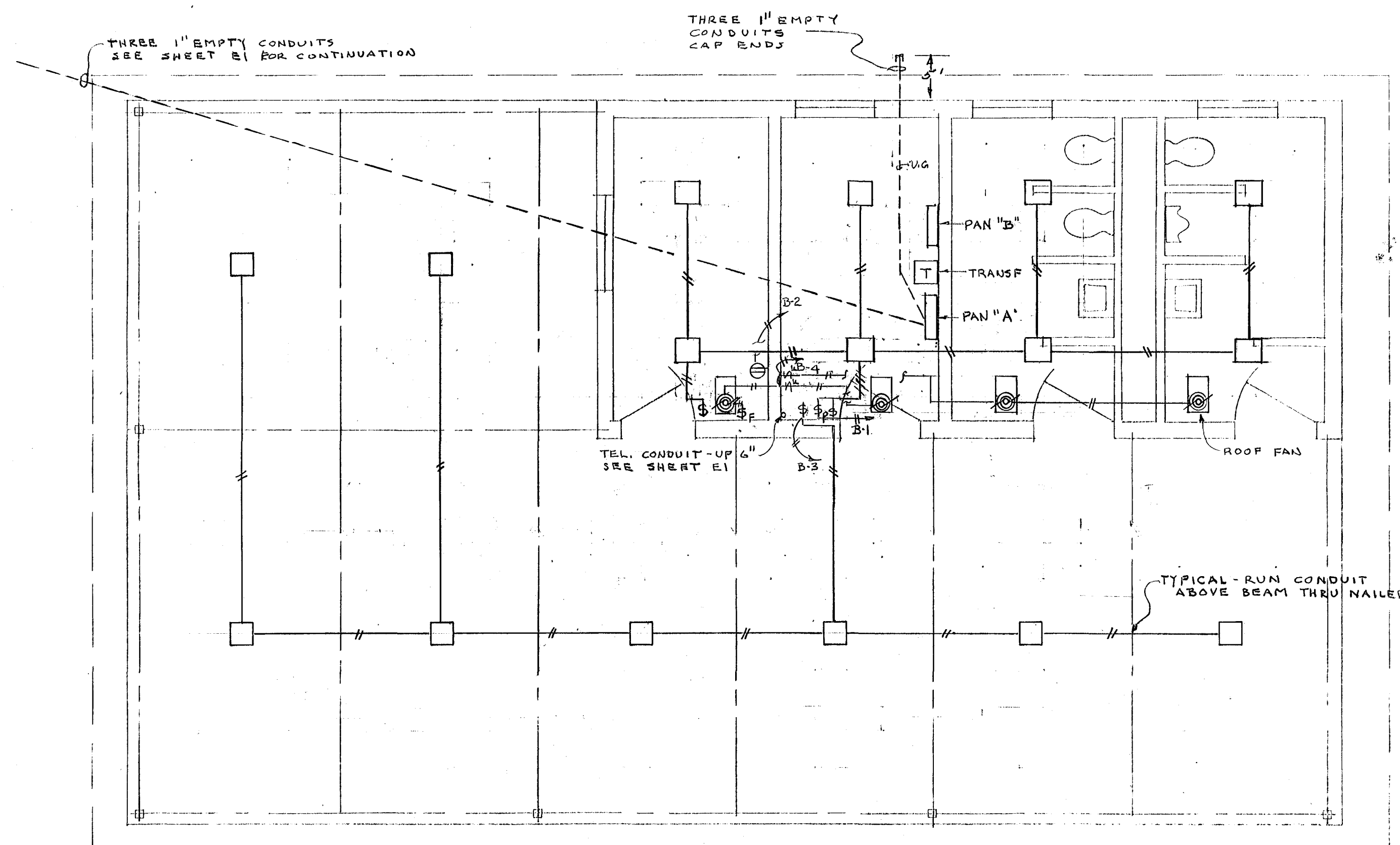
FLOOR PLAN ELECTRICAL
