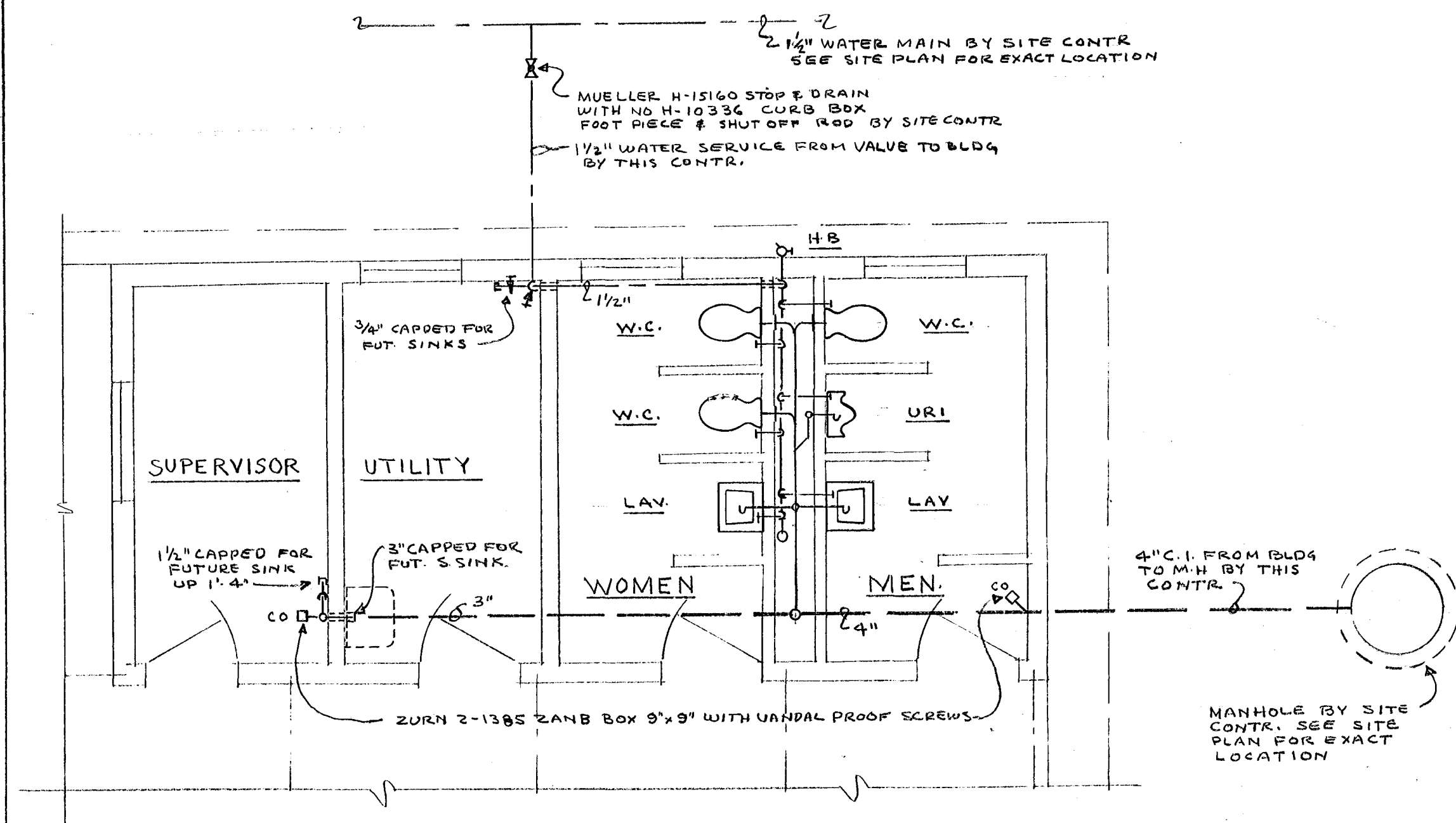
FLOOR PLAN PLUMBING
