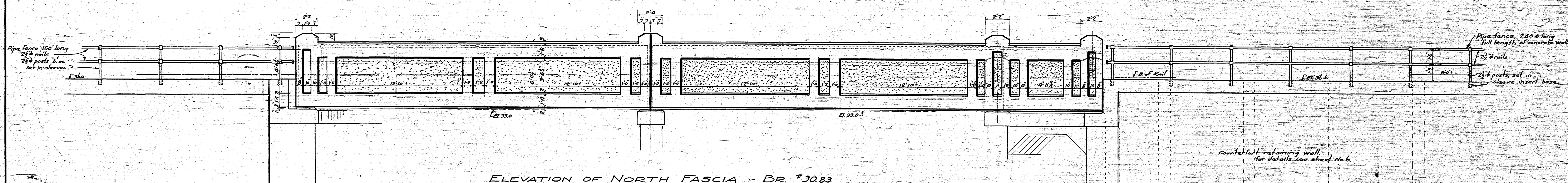
ELEVATION OF NORTH FASCIA - BR. #30.83
