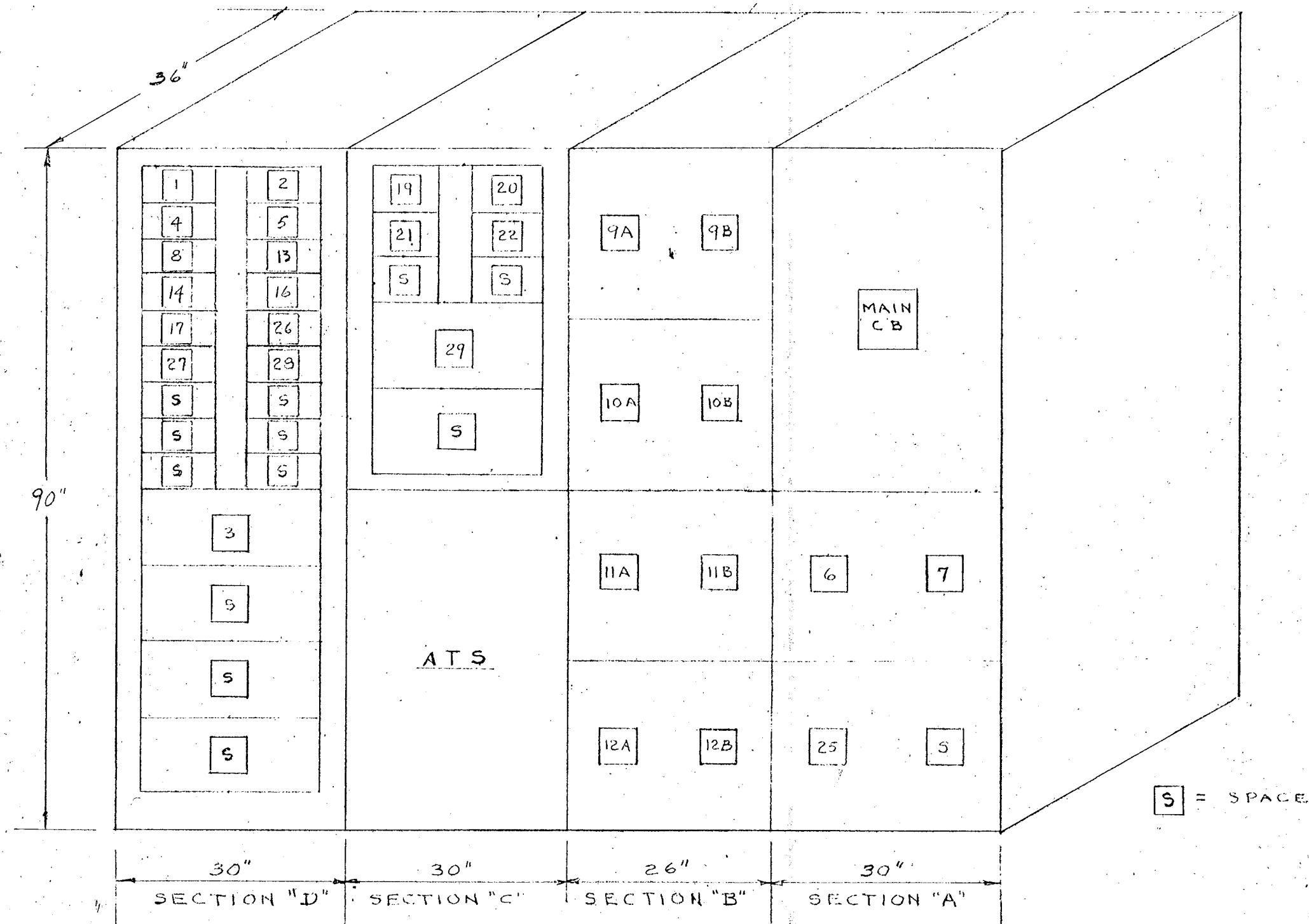
SWITCHBOARD LAYOUT
