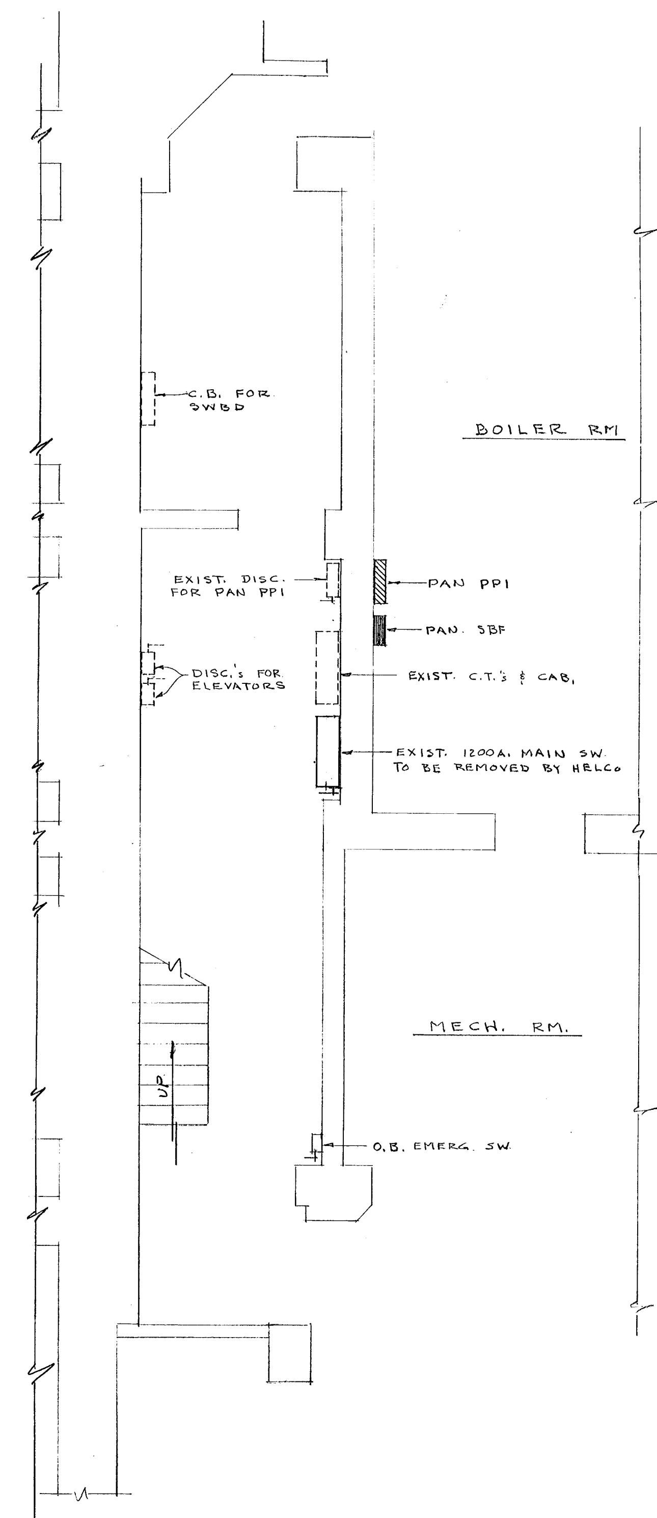
PARTIAL PLAN BOILER RM AREA
