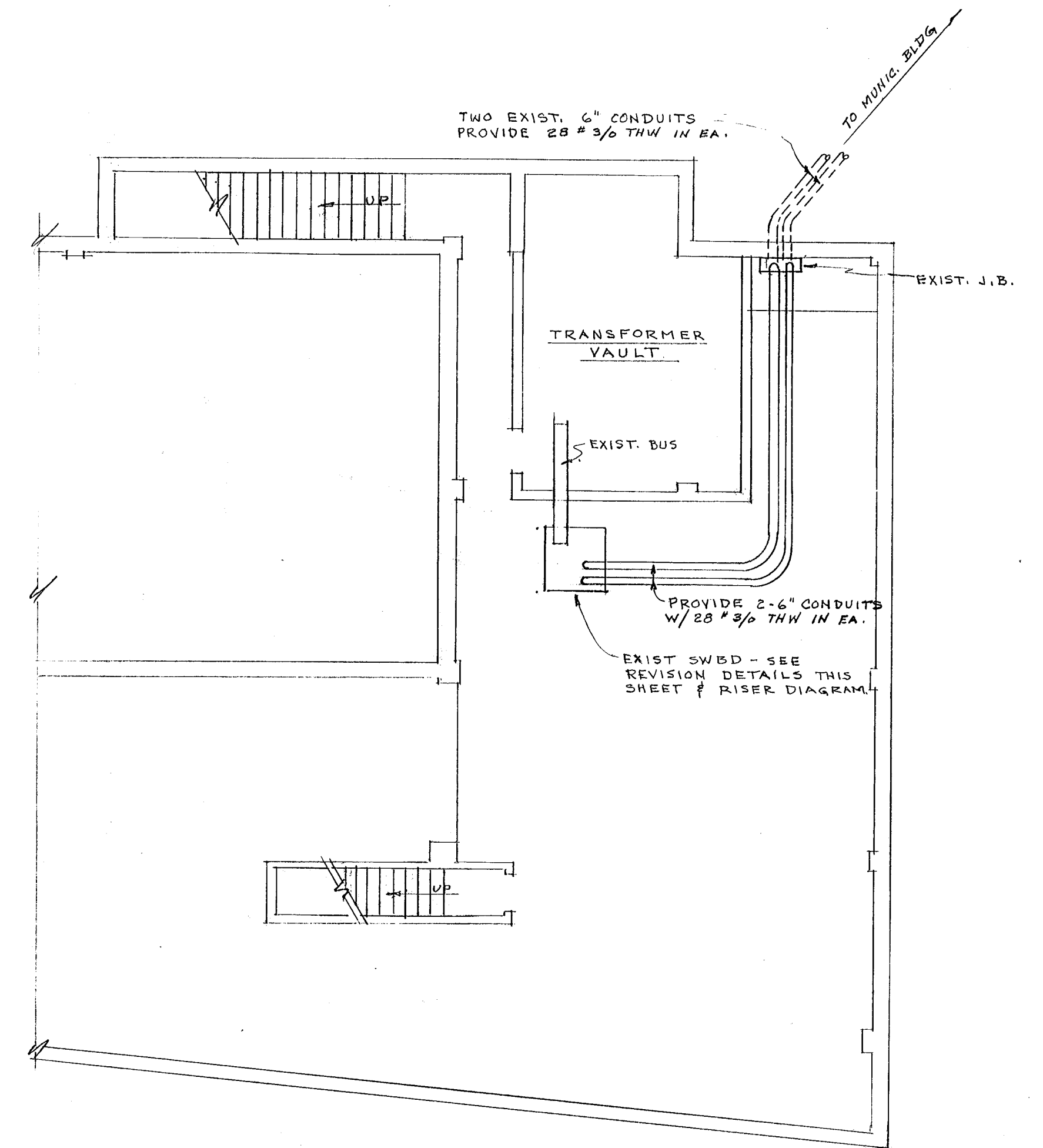
PARTIAL PLAN LIBRARY SUB-BASEMENT SCALE 1/8" = 1'-0"
