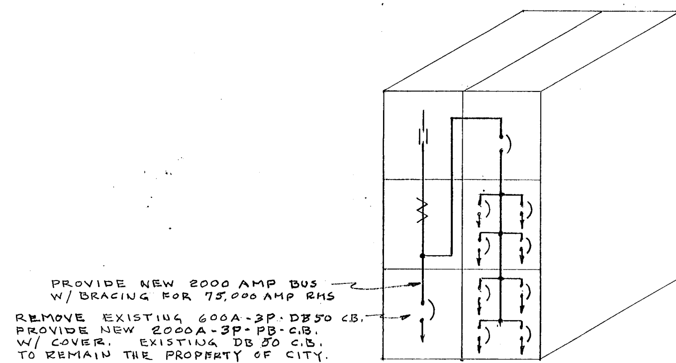
EXISTING LIBRARY SWITCHBOARD NO SCALE
