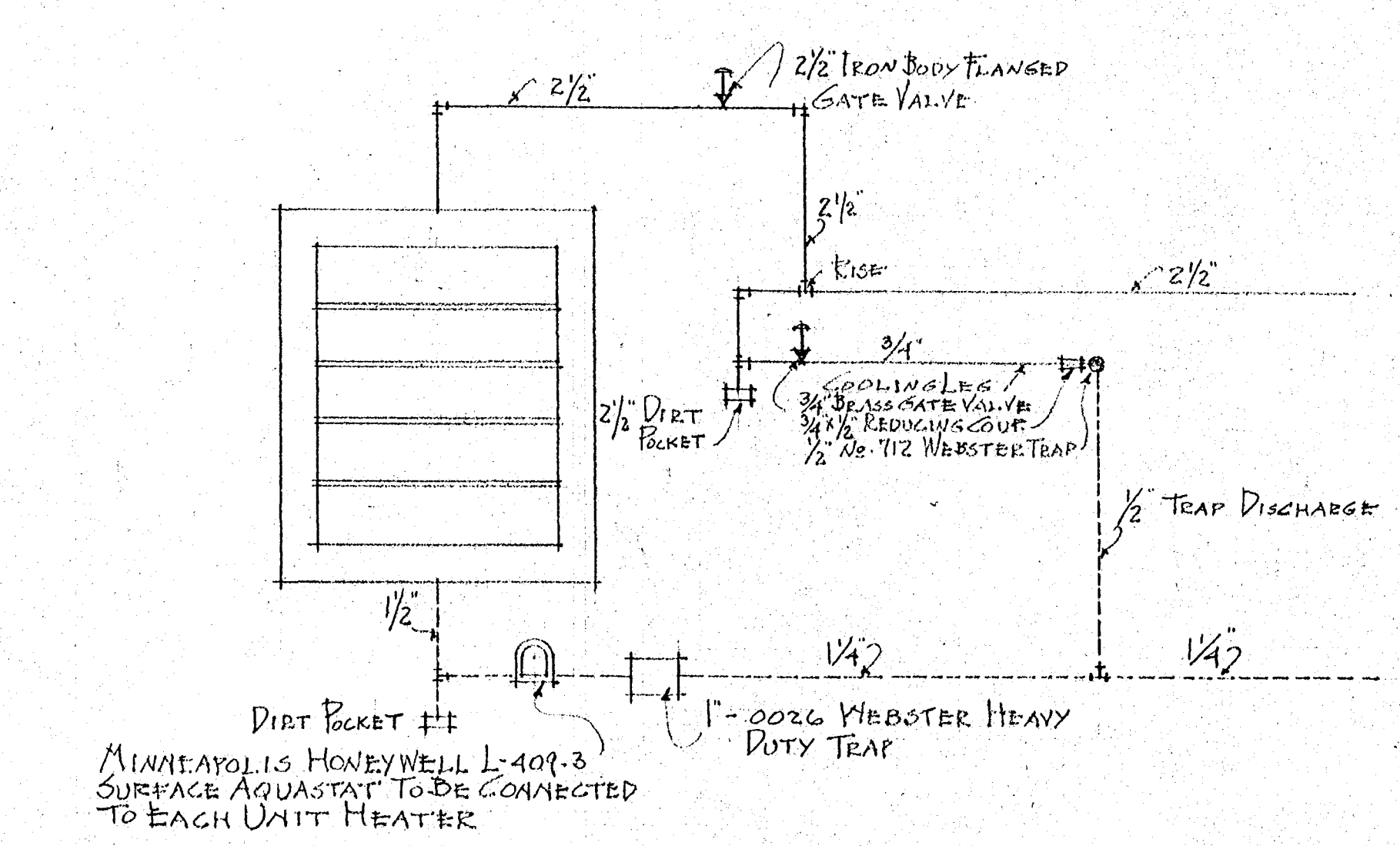
DETAIL OF PIPING CONNECTIONS TO UNIT HEATERS NUMBER ONE AND TWO
