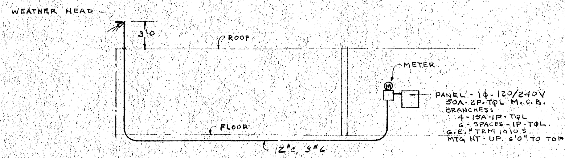
POWER RISER DIAGRAM NO SCALE
