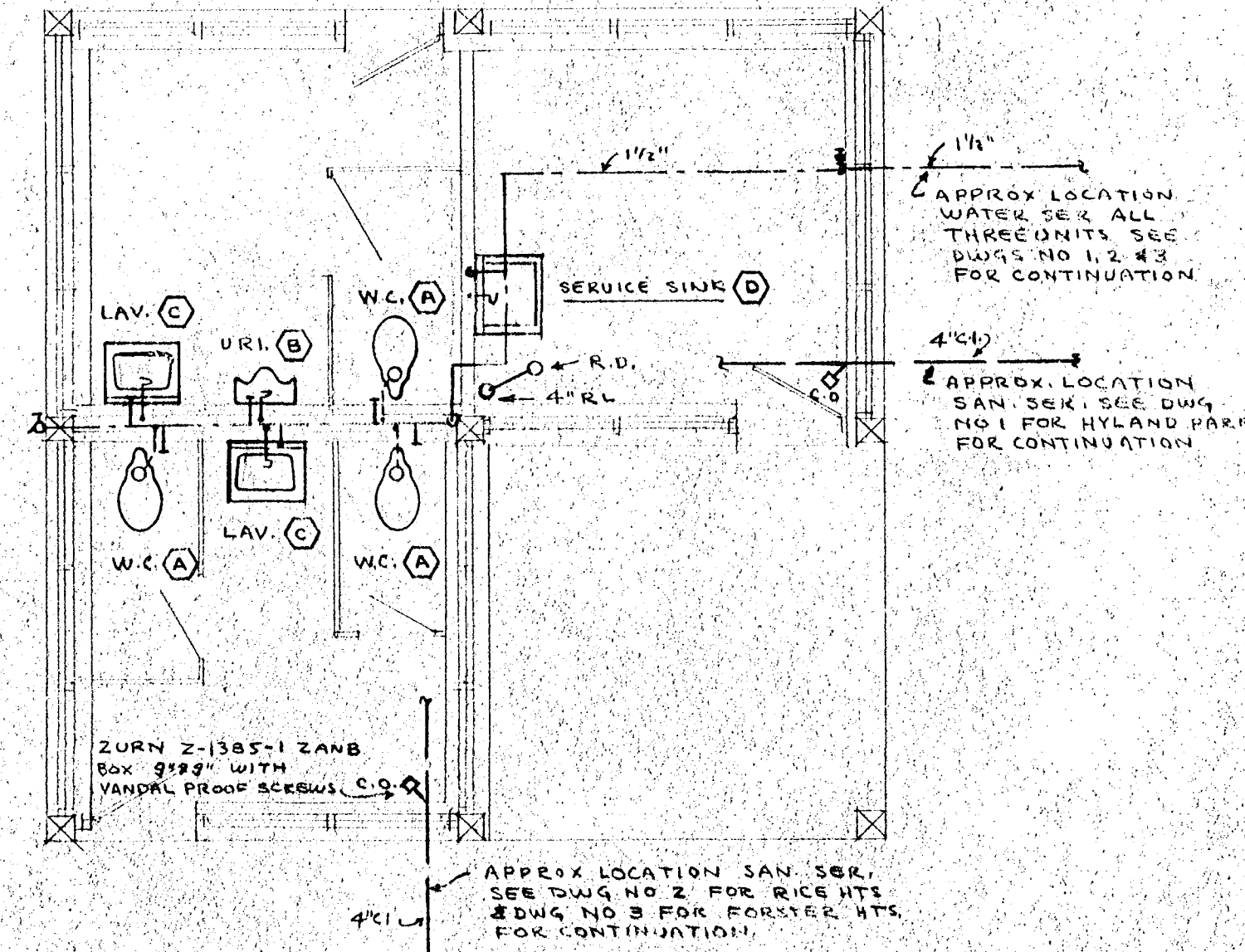
PLAN PLUMBING SCALE 1/4" = 1'-0"
